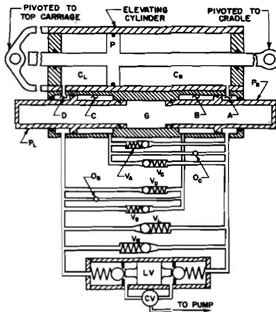
Figure 5. Hydraulic Elevating Mechanism—Power Type With Shock Absorber (Schematic)
