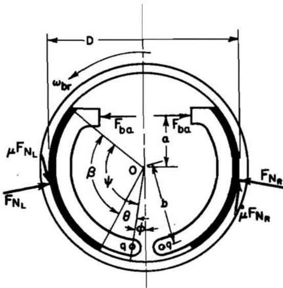
Figure 20. Brake With Applied Loads
