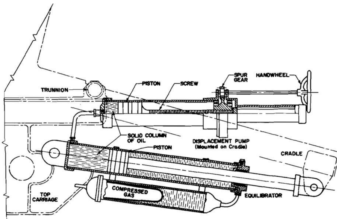
Figure 4. Hydraulic Elevating Mechanism—Manual Type (Combined With Equilibrator)
