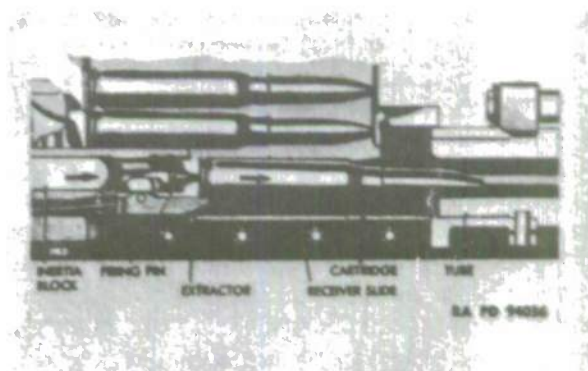
Figure 3-11. Bolt-type Breech Closure (Automatic Gun), Bolt Closing to Chamber the Cartridge
