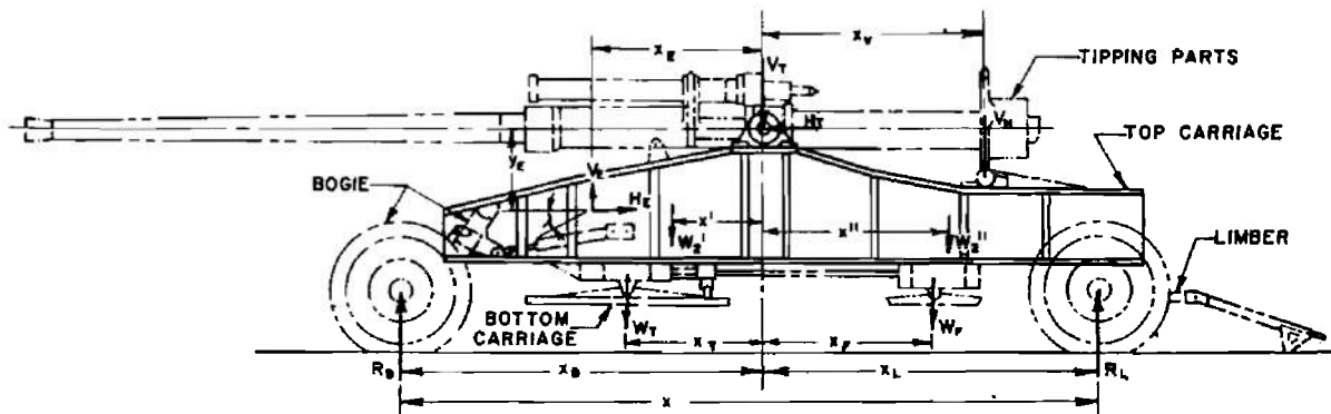
Figure 11. Top Carriage, Double Recoil Type, Transport Condition
