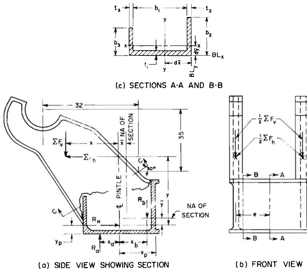
Figure 14. Composite Loads and Typical Section of Top Carriage
