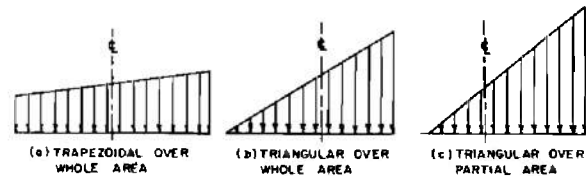
Figure 5. Types of Distributed Load on Thrust Bearing
