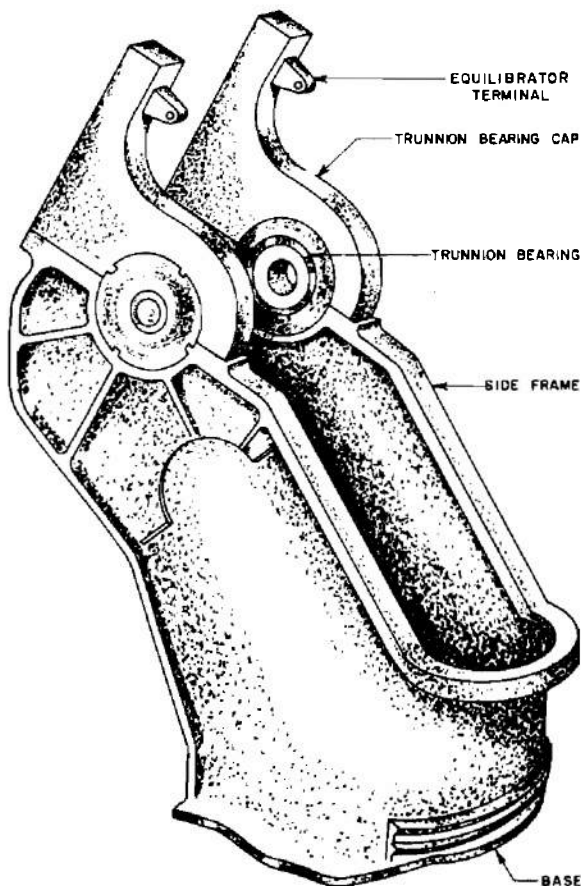
Figure 1. Typical Top Carriage Structure
