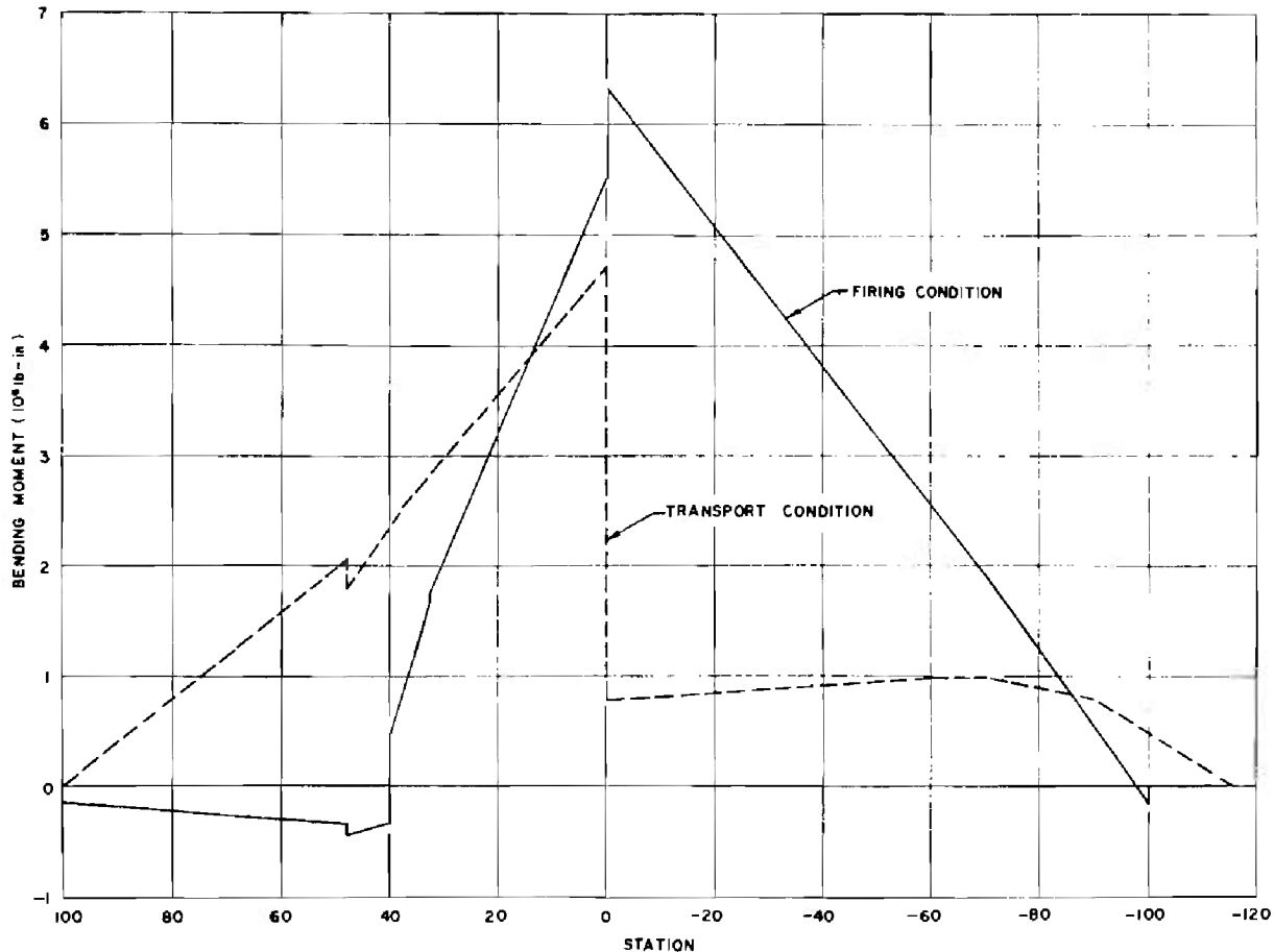
Figure 20. Design Bending Moment of Side Frame
