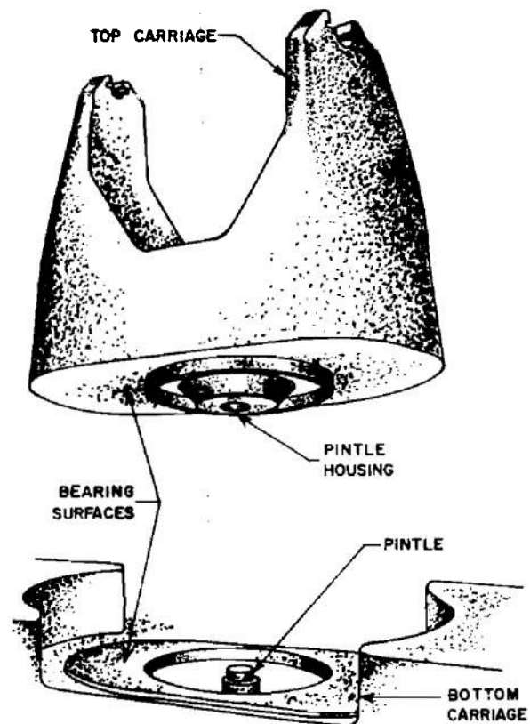
Figure 3. Smooth Surface Thrust Bearing
