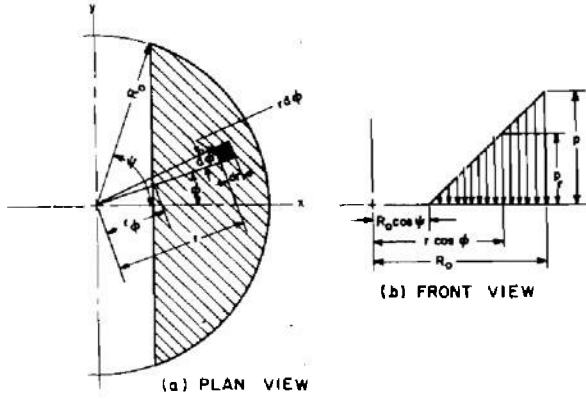
Figure 7. Loading Diagram of Circular Segment
