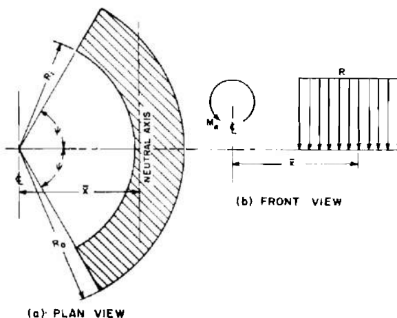
Figure 9. Uniform Load Distribution on Annular Sector
