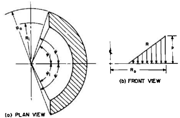
Figure 8. Loading Diagram of Annular Segment
