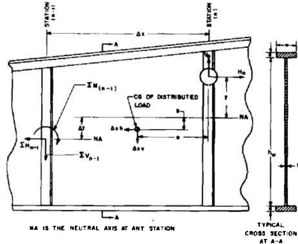
Figure 16. Load Analysis of a Side Frame Panel
