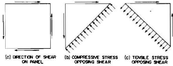
Figure 17. Stress Distribution of Panel
