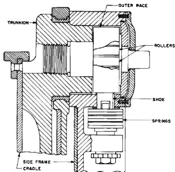
Figure 2. Trunnion Bearing (Antifriction Type)
