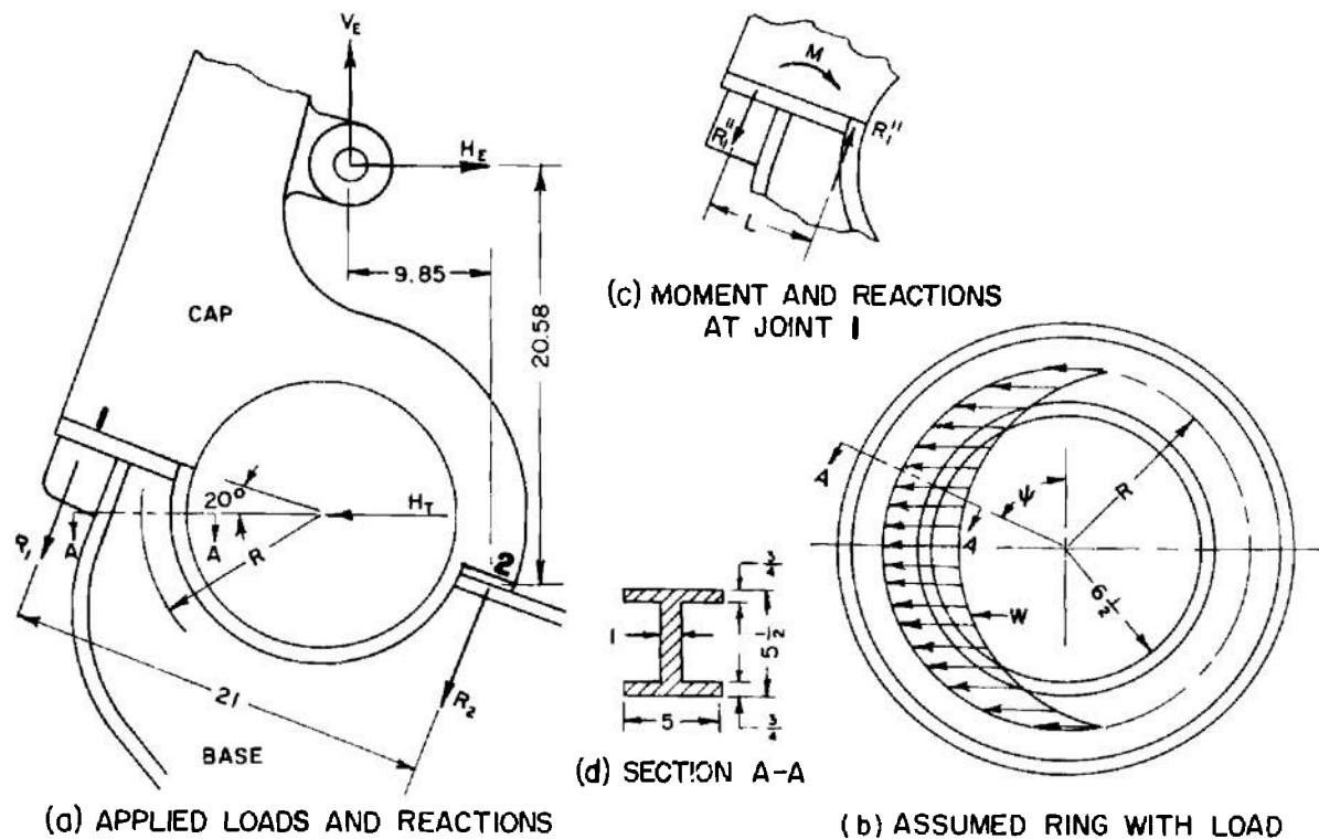
Figure 19. Trunnion Cap Loading Diagram
