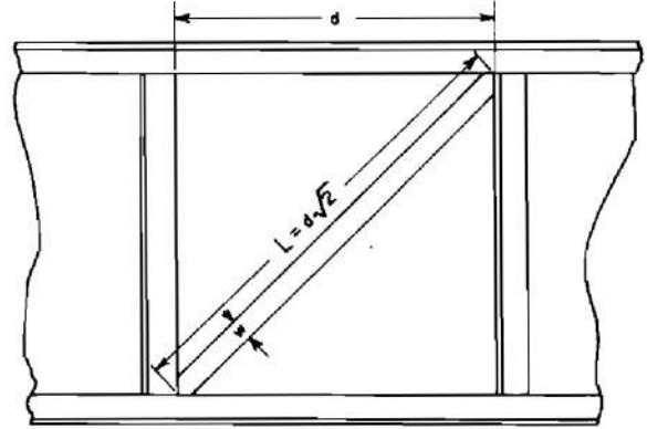
Figure 18. Stiffener Spacing Based on Column Analogy
