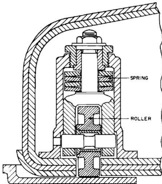
Figure 4. Traversing Roller Assembly
