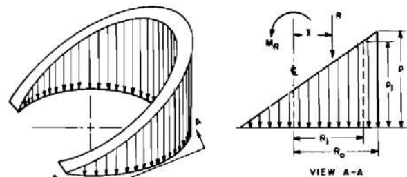
Figure 6. Triangular Load Distribution on Annular Segment
