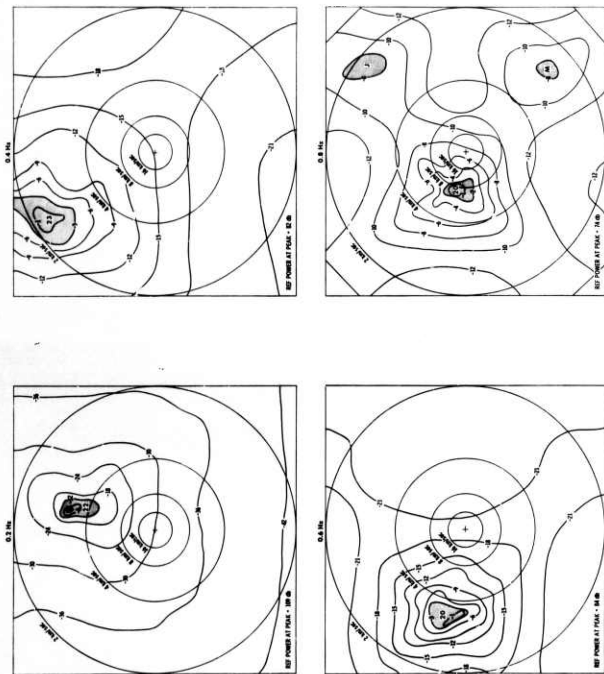
Figure II-5. High-Resolution Frequency-Wavenumber Spectra at OONW: 29 January 1965 Noise Sample
