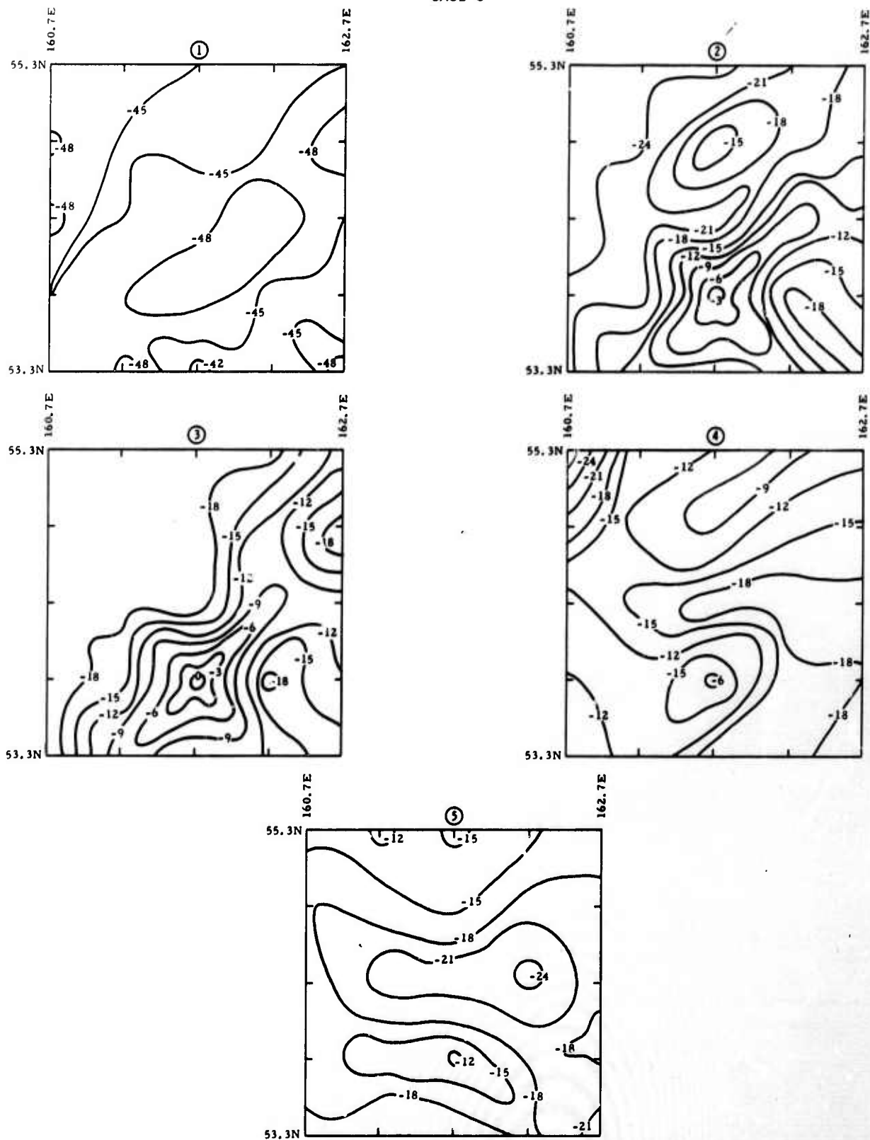
Figure V-13. Beamsteered Plots for Five Time Traces for Case C
