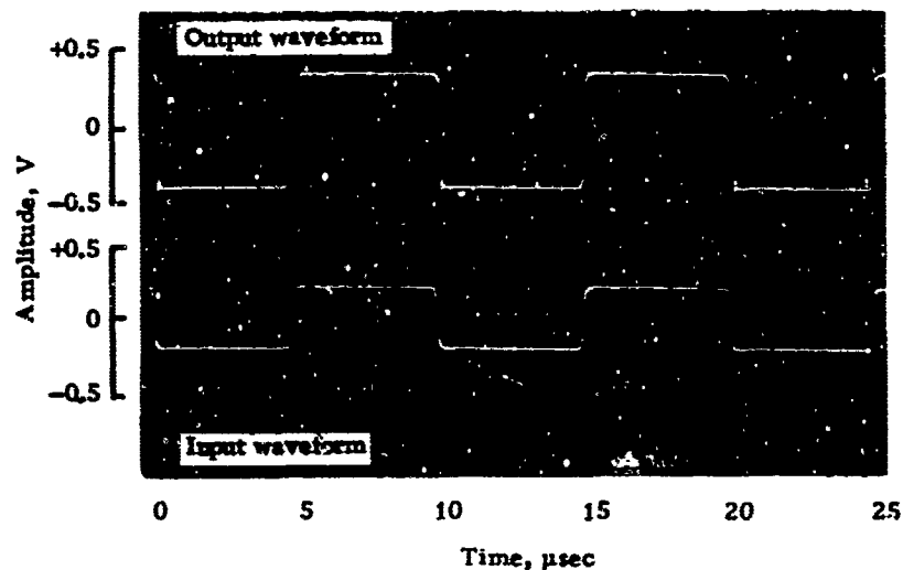
FIG. 6. 100-kHz Square-Wave Response.
