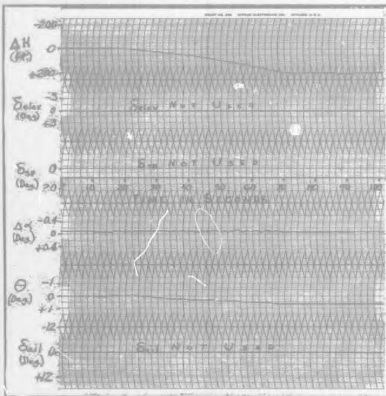
Fig. 6-17. Flight Condition One, Basic Aircraft With Turbulence, Hands Off Controls, TDF Simulation
