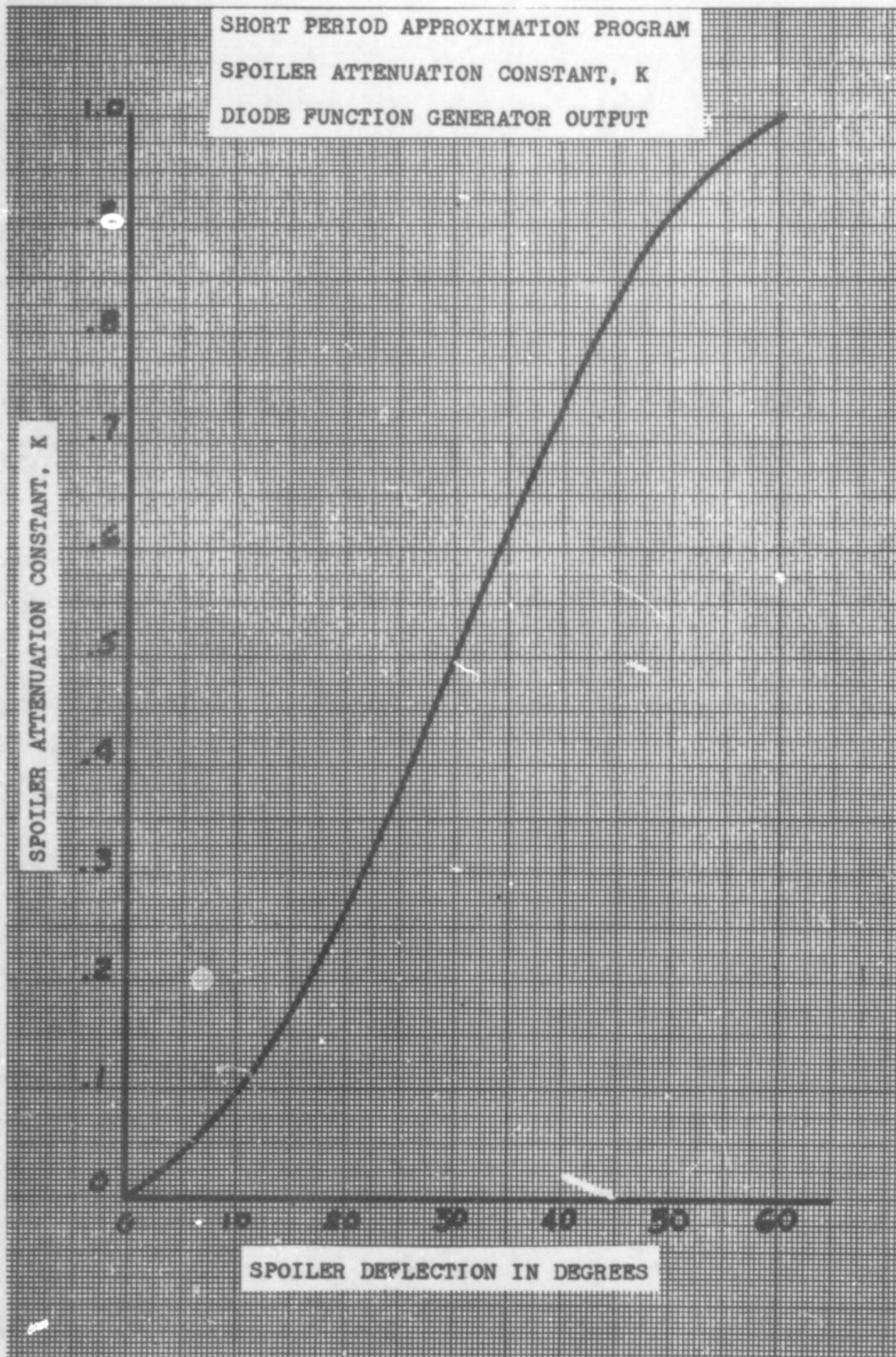
Fig. 3-1. Spoiler Attenuation Constant
