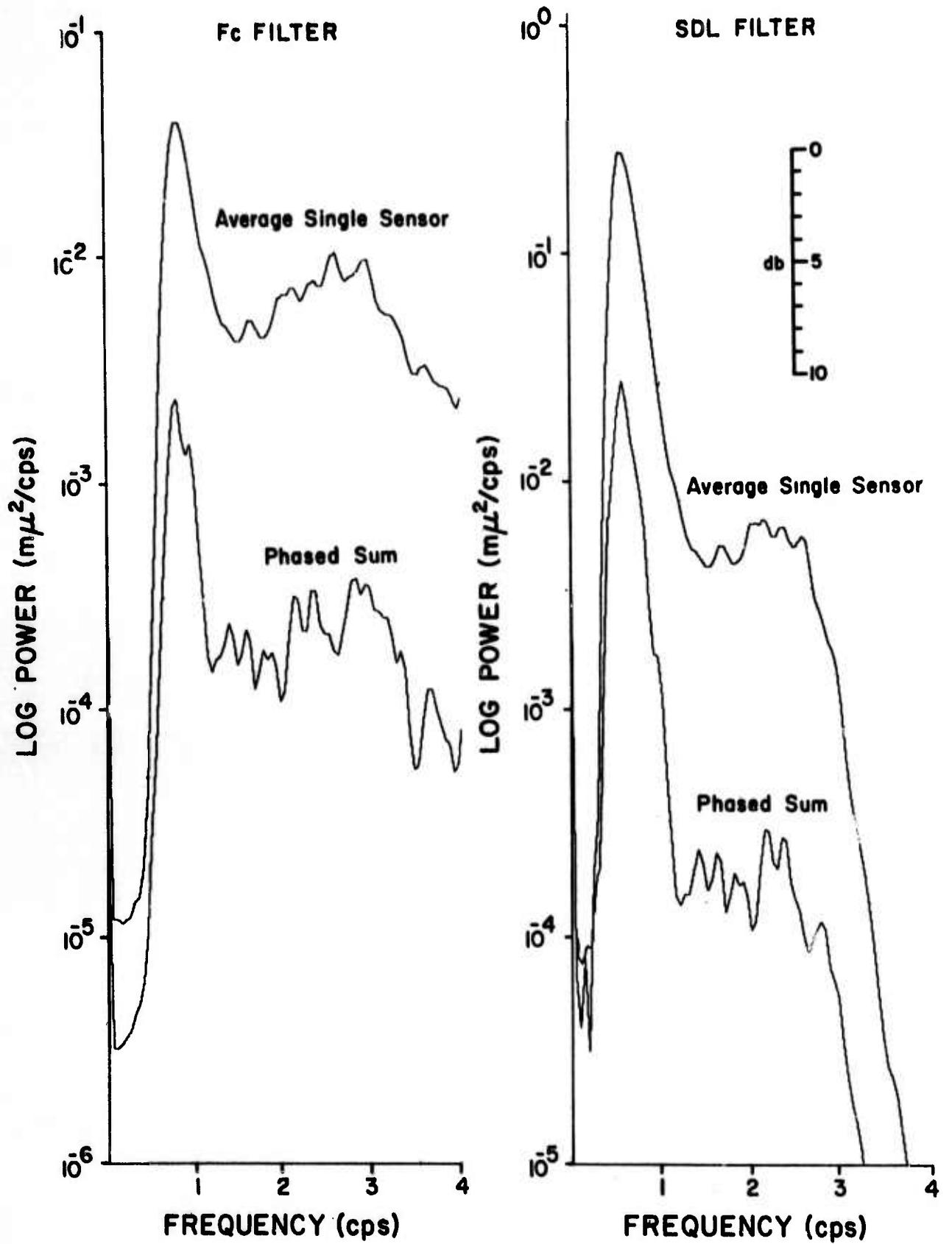
Figure 7.. Noise power spectra, Tunisia, 25 February 1968.
