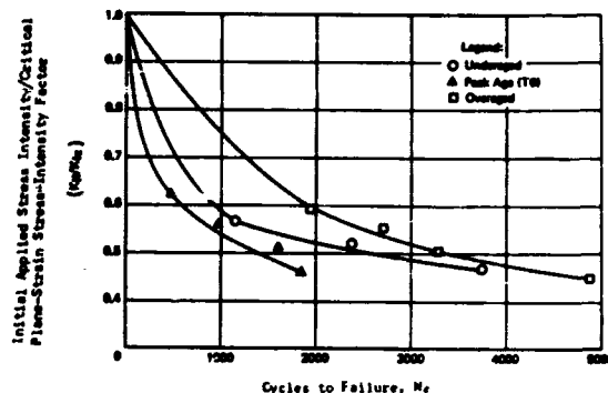
FIGURE 2. COMPARISON OF K_{I1}/K_{IC} VERSUS FATIGUE CYCLES TO FAILURE FOR 0.63-INCH-THICK 7079 UNDER-AGED, PEAK-AGE (T6), AND OVERAGED MATERIALS (5)
