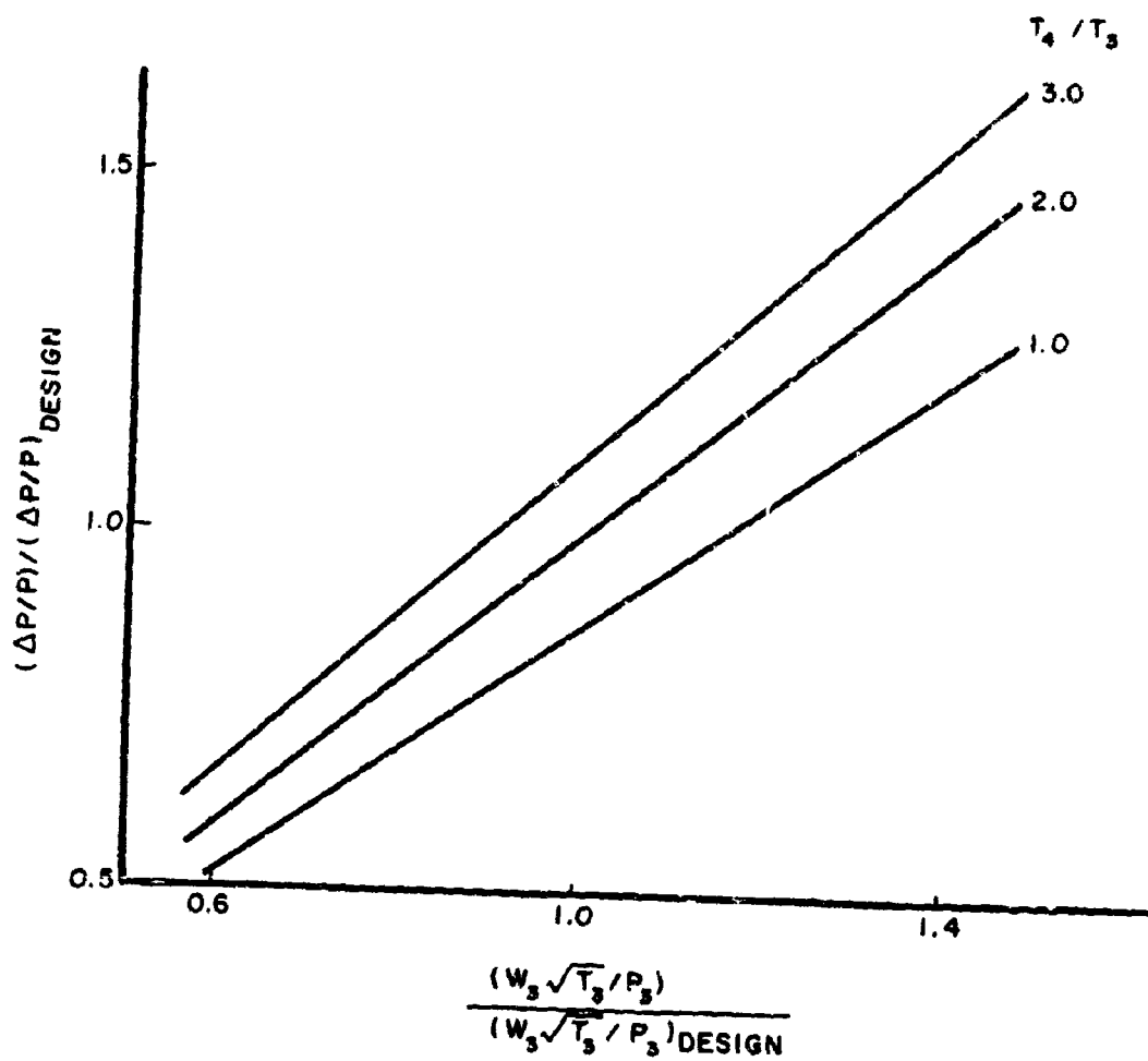
Figure 24. 12 Pressure Ratio Turbojet Combustor Characteristics
