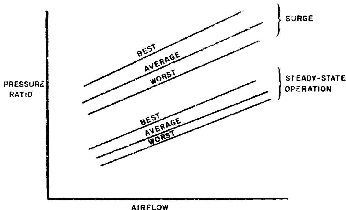
Figure 19. Effect of Manufacturing Tolerances
