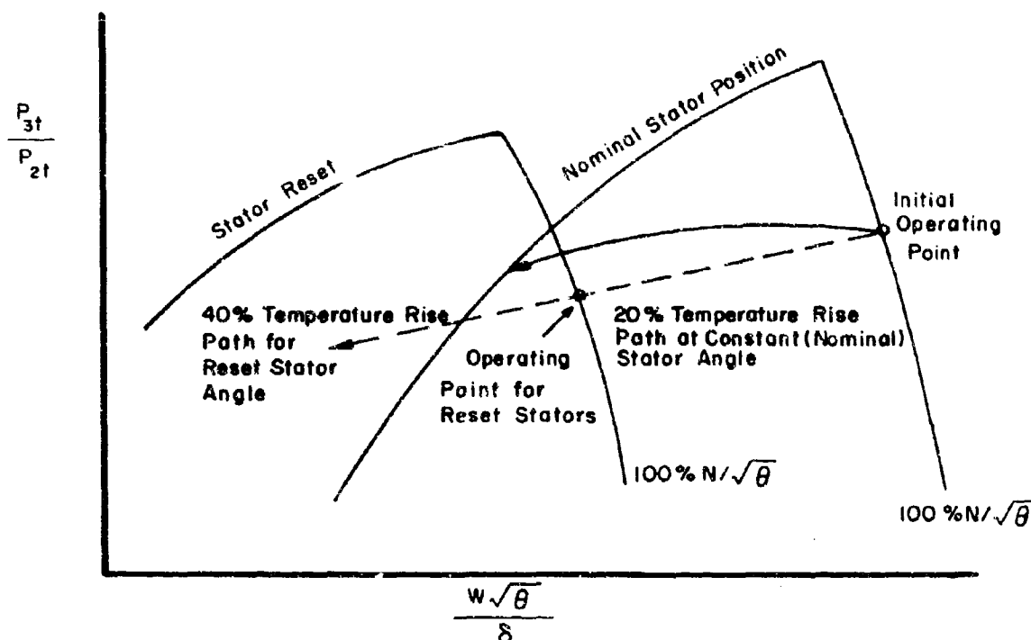
Figure 20. Stator Angle Shift for Surge Control (Rapid Inlet Temperature Rise)
