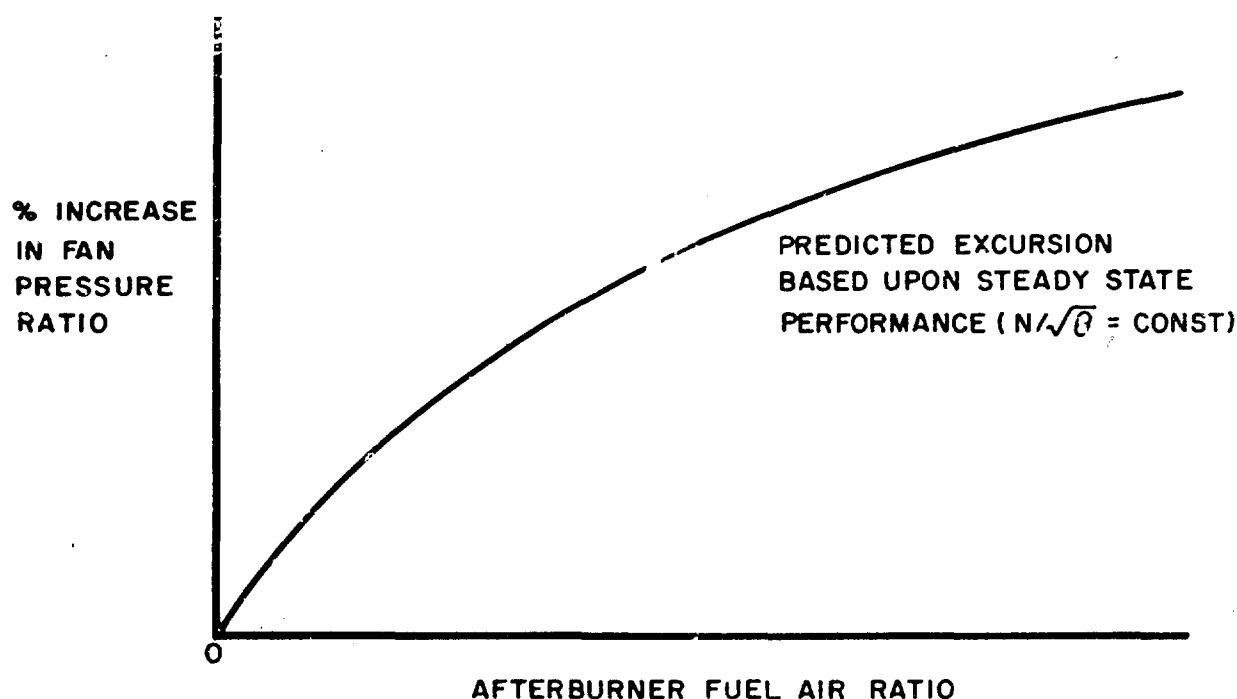
Figure 18. Effect of A/B Light on Fan Pressure Ratio
