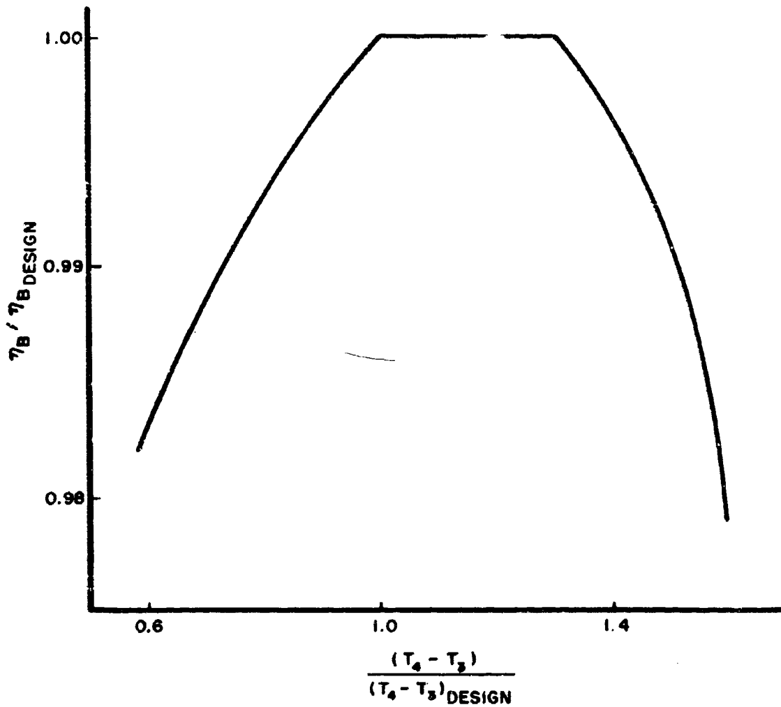
Figure 25. 12 Pressure Ratio Turbojet Combustor Characteristics
