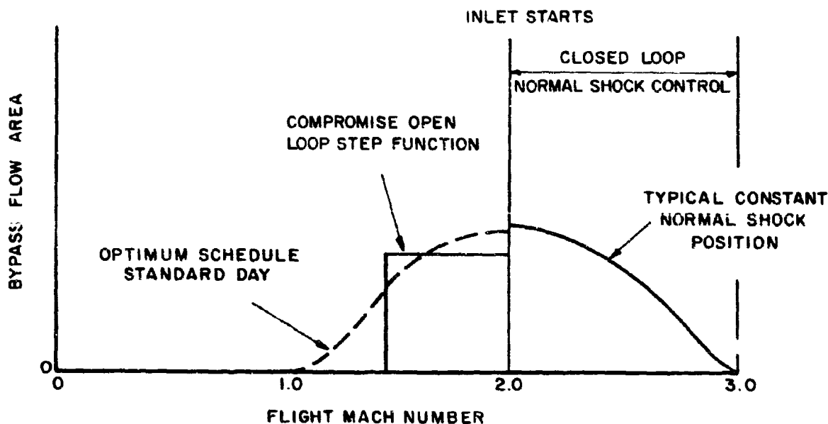
Figure 12. Bypass Control Functions
