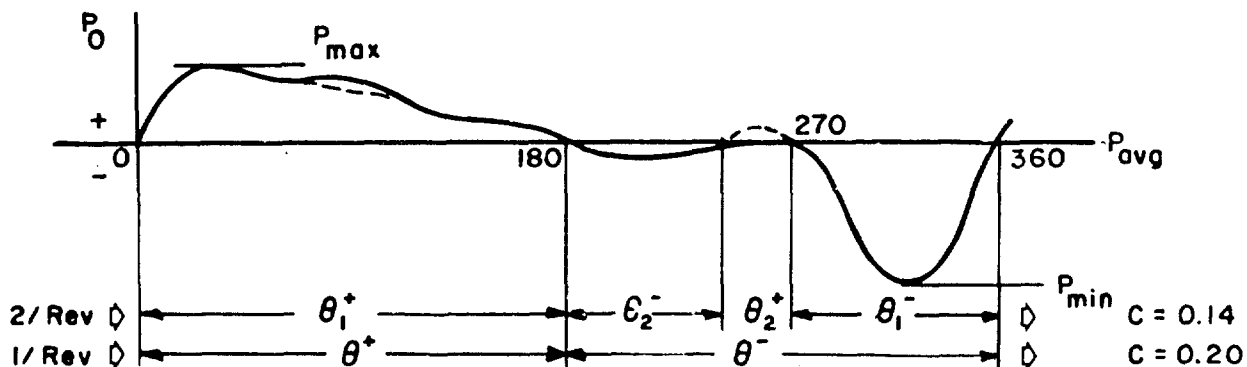
Figure 4. Circumferential Pressure Variation
