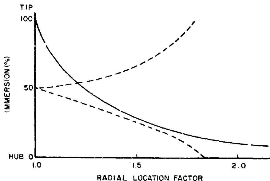
Figure 7. Radial Location Factors
