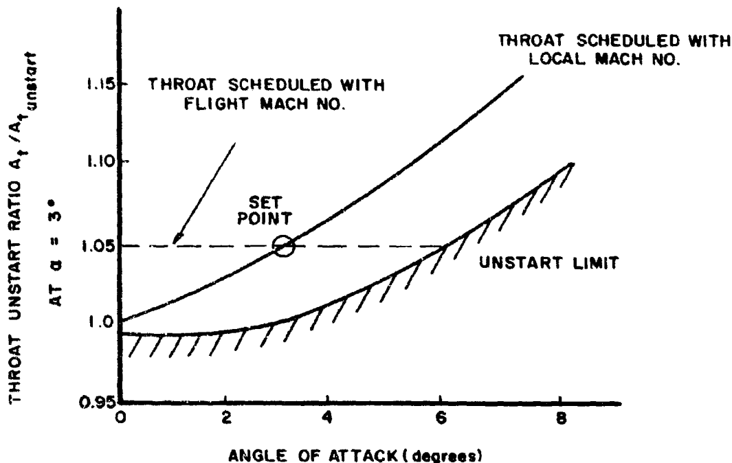
Figure 10. Effect of Aircraft Pitch Attitude on Unstart Throat Margins at Mach 3.0
