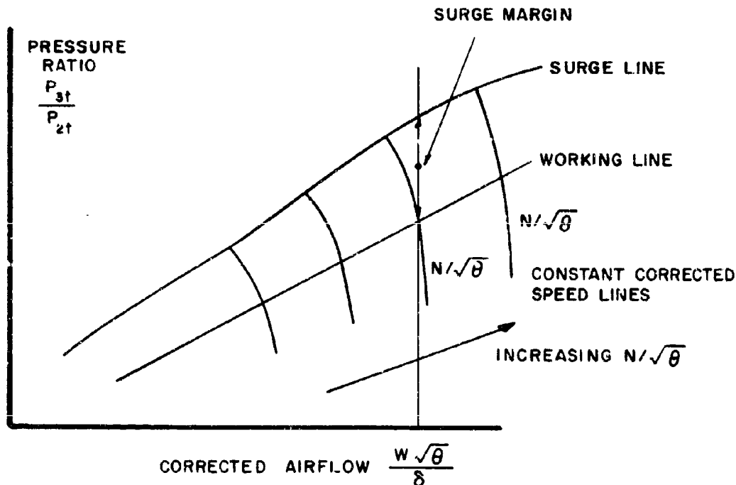
Figure 16. Typical Compressor Characteristic Map
