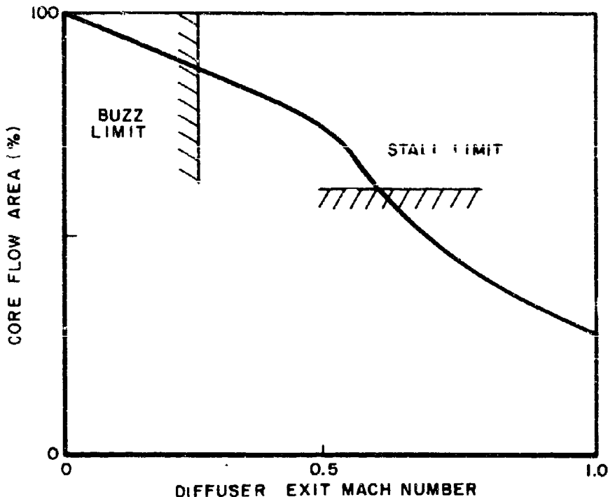
Figure 1. Typical Inlet/Engine Stability Range
