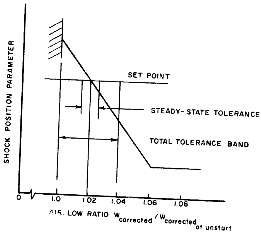
Figure 13. Normal Shock Parameter at Maximum Flight Speed
