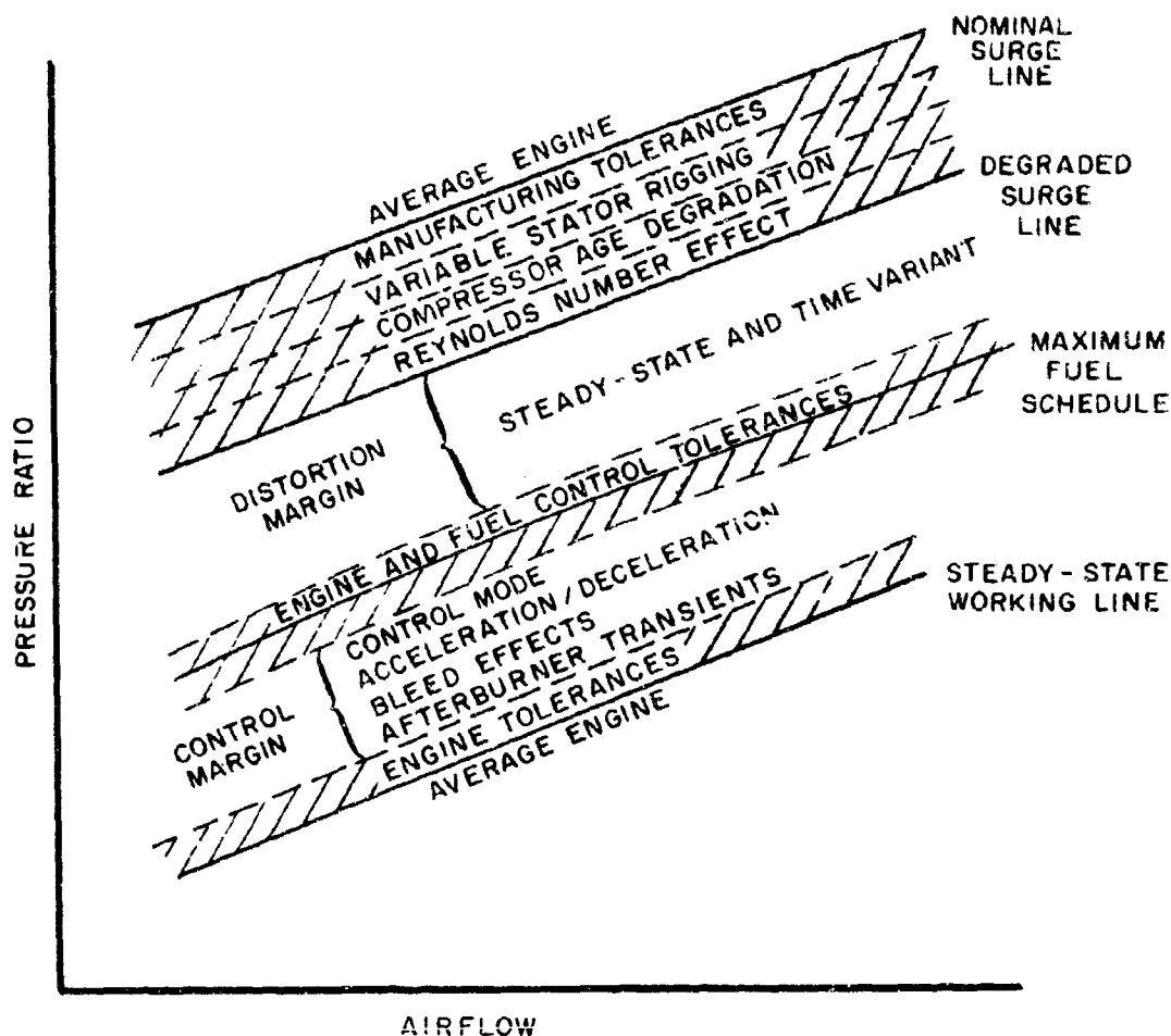
Figure 23. Cumulative Representation of Degrading Factors on a Compressor Performance Map
