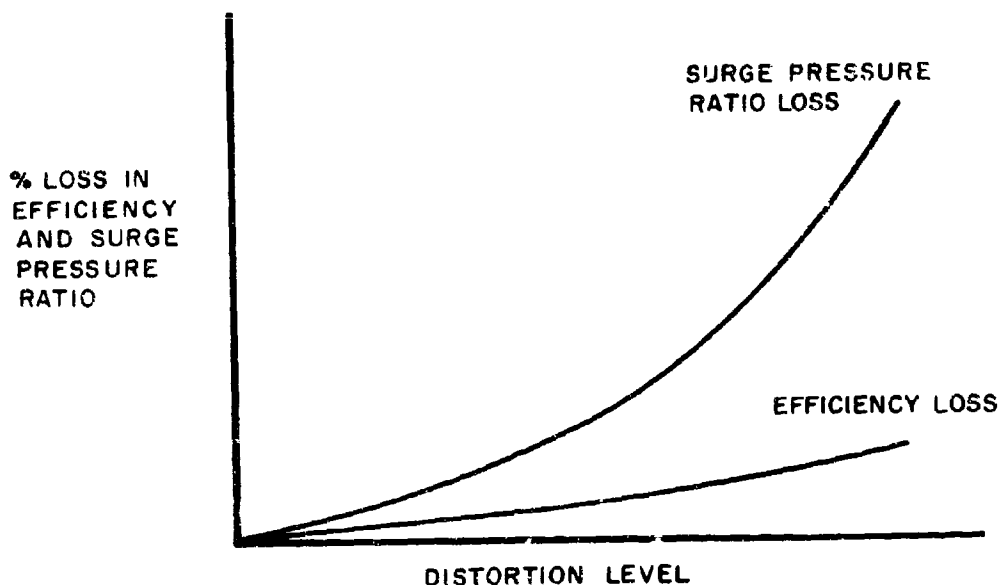
Figure 21. Distortion Effect on Compressors
