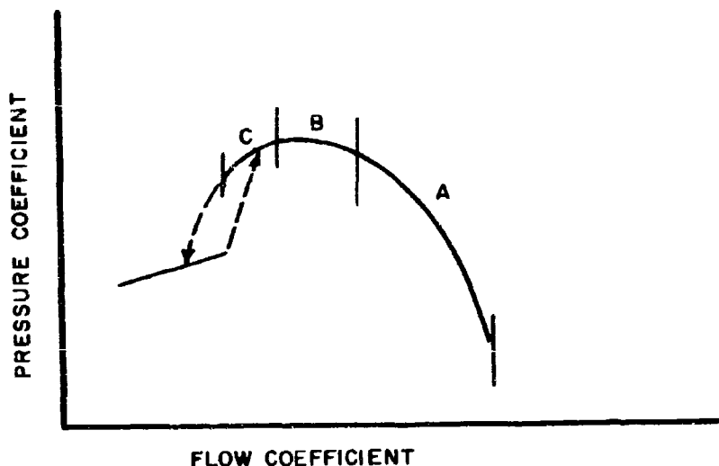
Figure 2. Typical Compressor Stage Characteristic
