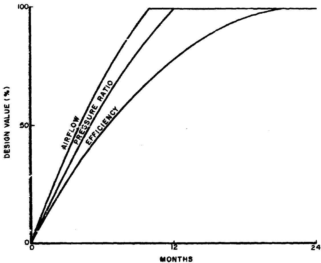
Figure 28. Advanced Compressor Development General Performance History
