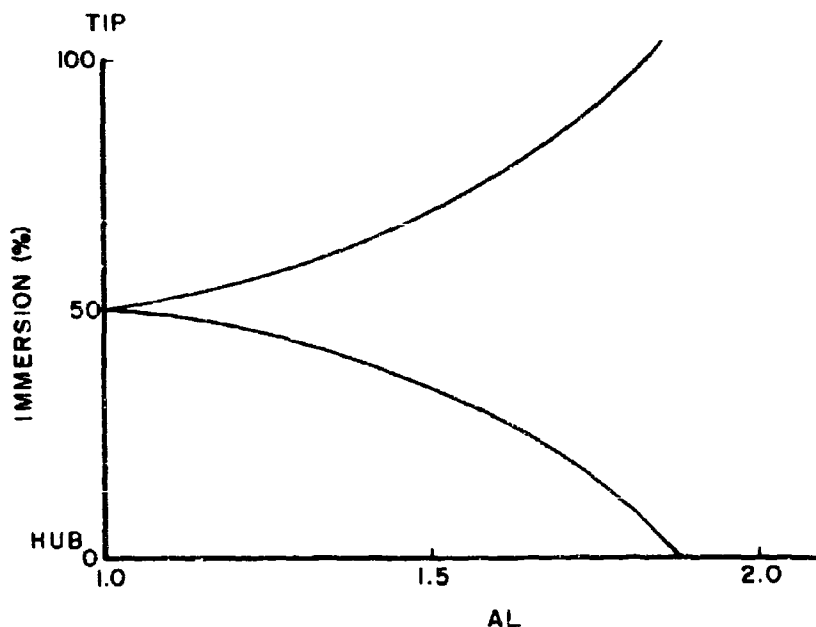
Figure 6. Radial Weighting Factor
