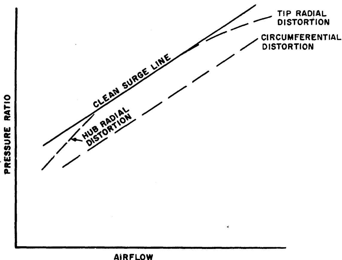
Figure 33. General Compressor Surge Line Shift
