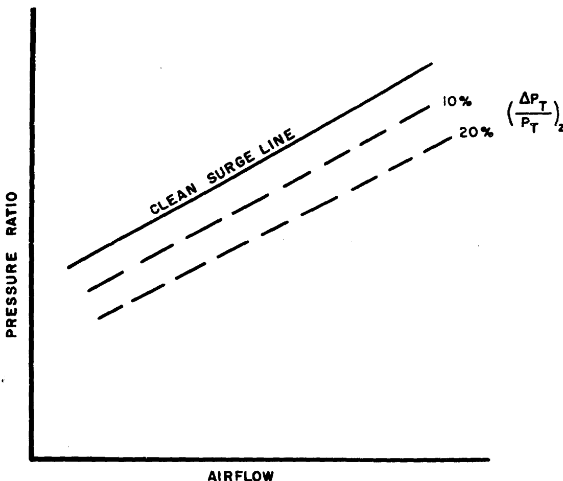
Figure 34. Compressor Surge Line Shift With Varying Levels of Circumferential Distortion
