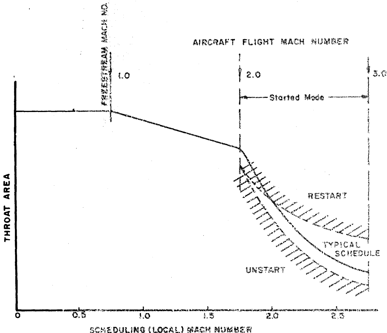
Figure 8. Throat Control Function
