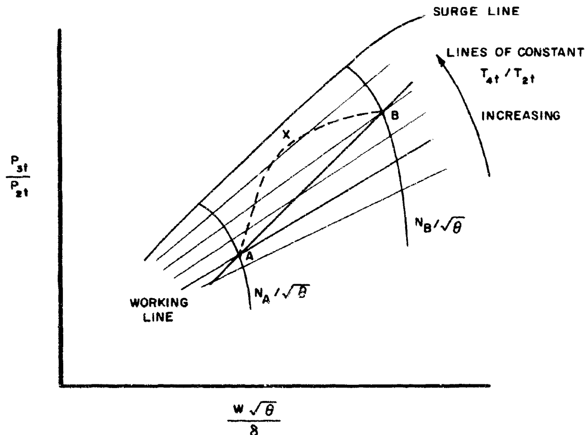
Figure 17. Effect of Acceleration
