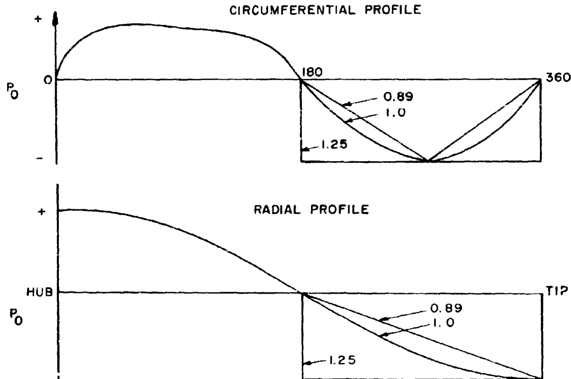
Figure 5. Circumferential and Radial Profiles
