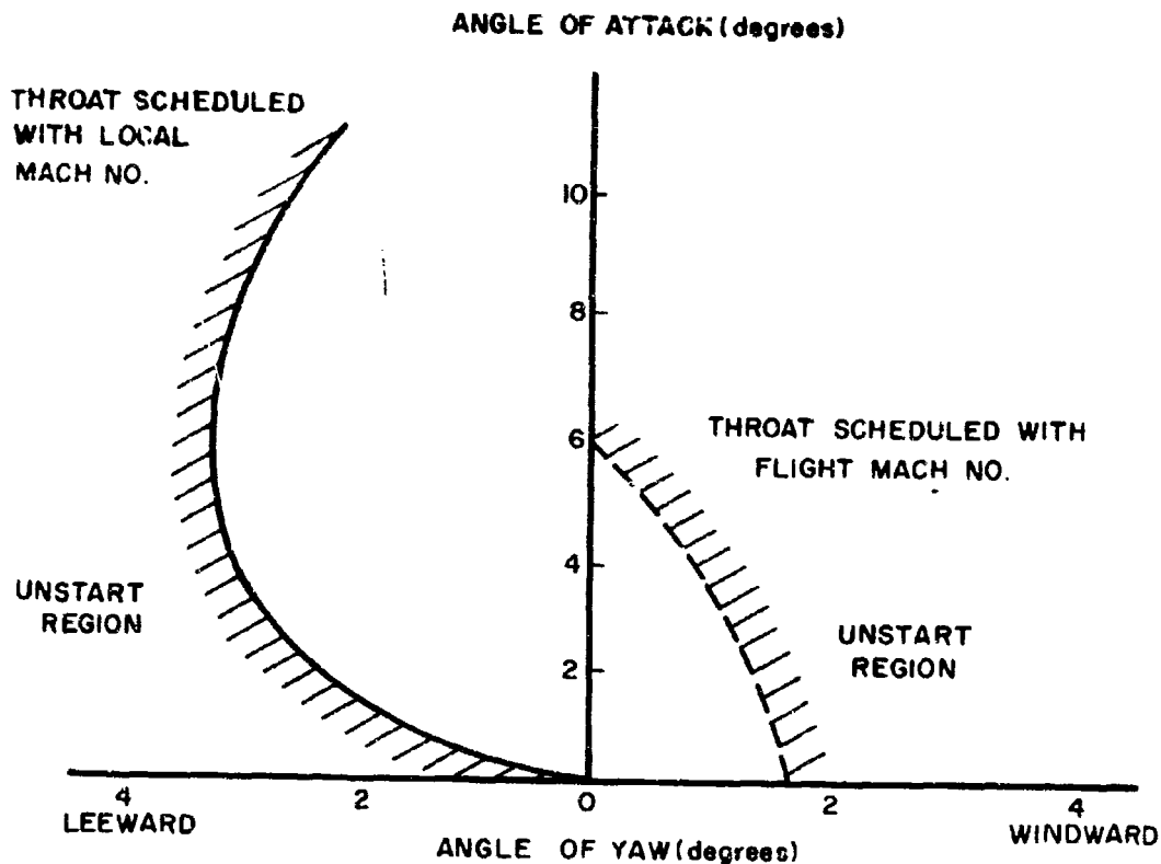
Figure 11. Effect of Aircraft Yaw Attitude on Unstart Throat Margins at Mach 3.0
