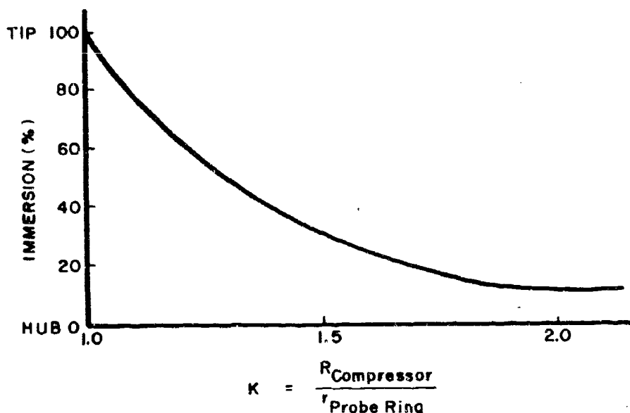
Figure 3. Radial Location Factor
