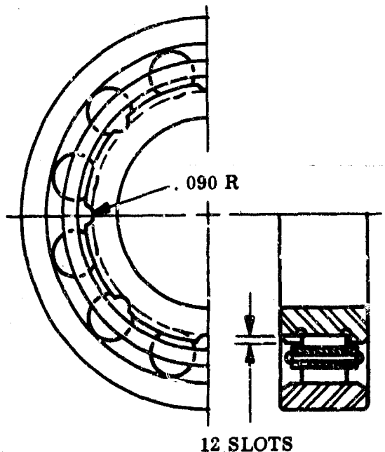
Figure 7. Test Bearing R-2 and R-2 Modified
