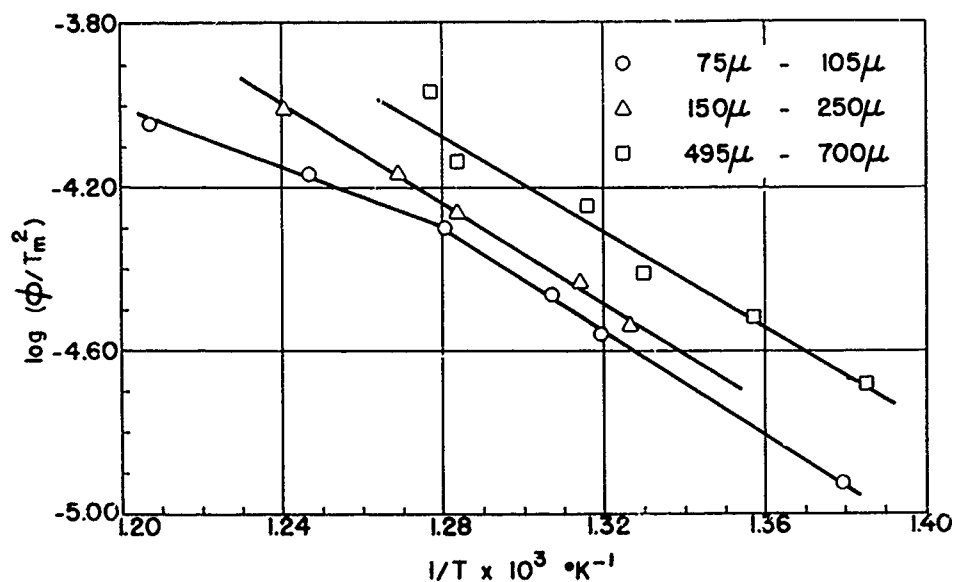
FIG. 2.18. Plot of \text{Log}(\phi/T_m^2) Versus 1/T for the Decomposition of Pure AP: Reaction of the second DTA exotherm. Particle sizes 75 \mu - 105 \mu , 150 \mu - 250 \mu , and 495 \mu - 700 \mu .
