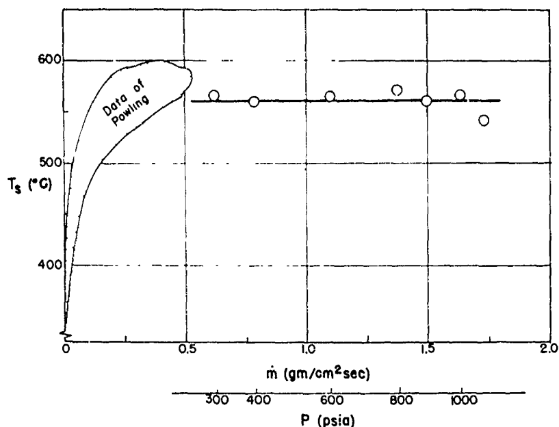
FIG. 2.31. Calculated Temperature of the Solid Surface as a Function of Pressure and Mass Burning Rate (Compared with the Data of Powling (Ref. 52)).
