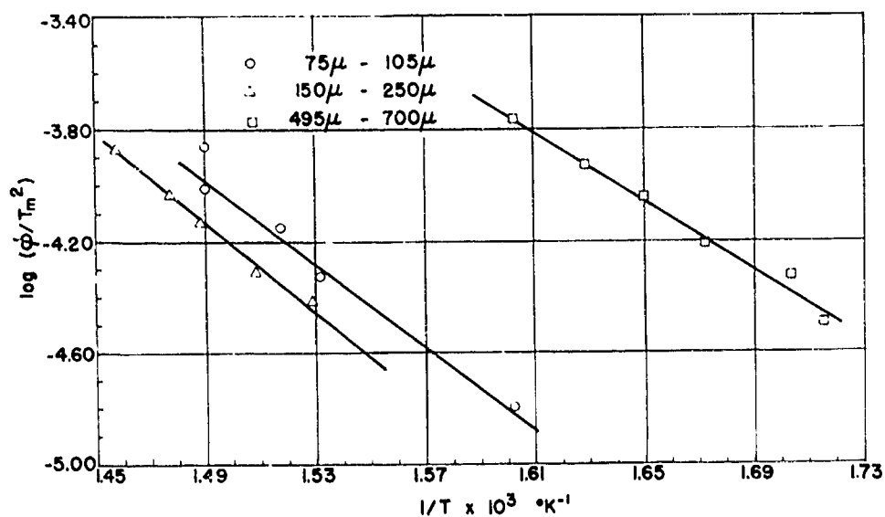
FIG. 2.17. Plot of \text{Log}(\phi/T_m^2) Versus 1/T for the Decomposition of Pure AP: Reaction of the first DTA exotherm. Particle sizes 75 \mu - 105 \mu , 150 \mu - 250 \mu , and 495 \mu - 700 \mu .
