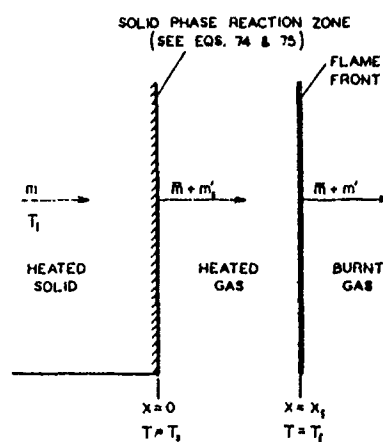
Figure 3. Model Used in Refs. 1, 30, 39, 40.
