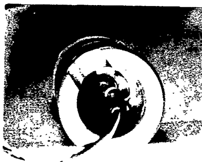
PHOTO 9 FORWARD INSTRUMENTED AXLE ASSEMBLY - STOW SYSTEM - END VIEW SHOWING PLACEMENT OF STRAIN GAGES .
