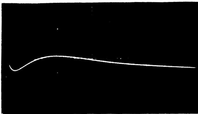
0.1 V/div 100 μs/div Conductor-to-Ground Voltage
