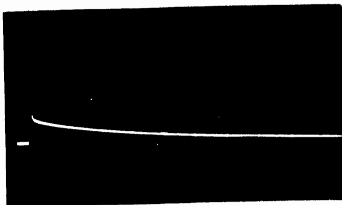
10 V/div 10 μs/div Conductor-to-Ground Voltage
