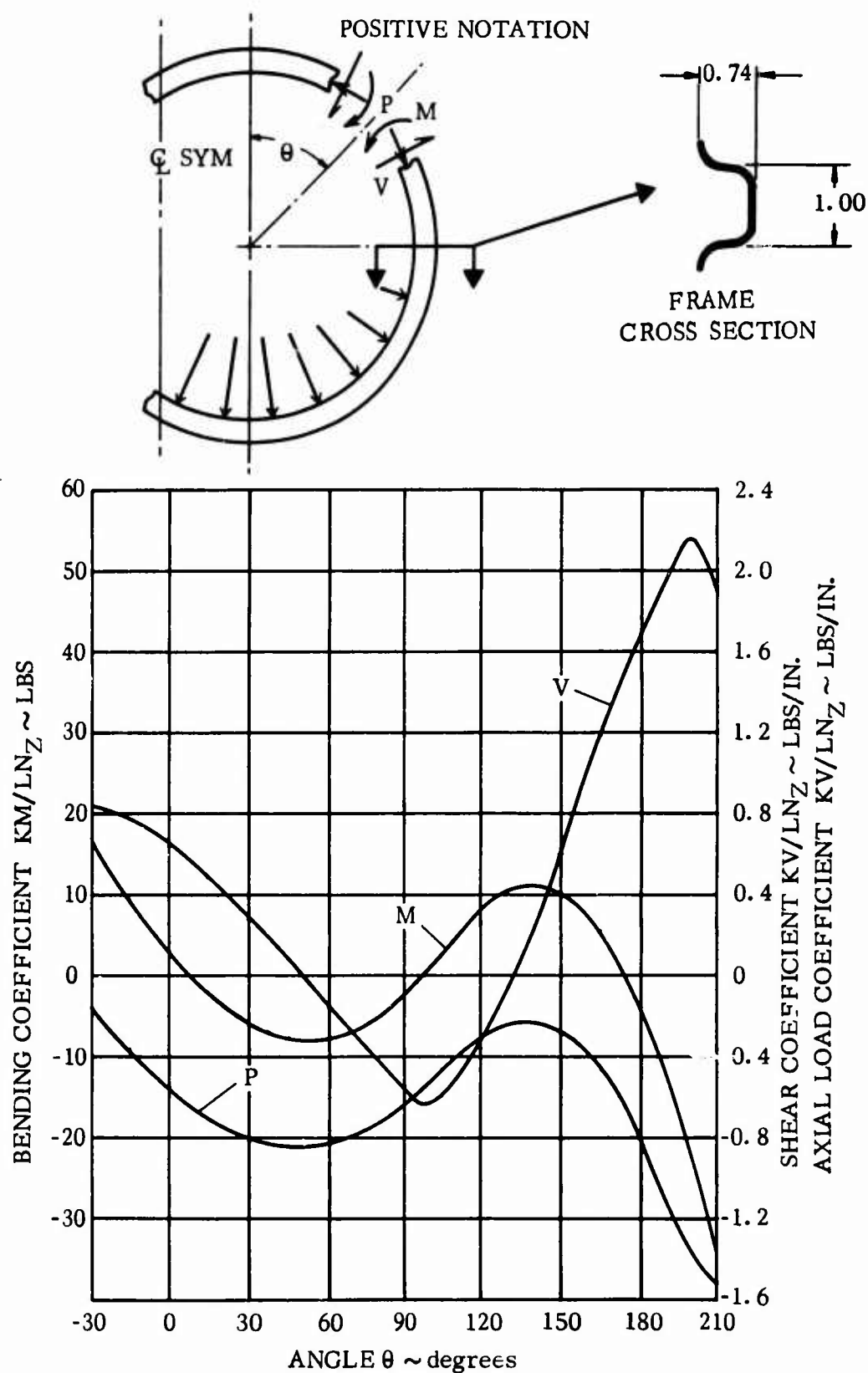
Figure 22. Loading of Intermediate Frames - Half-Full Fuel Condition
