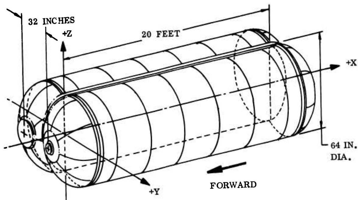
Figure 6. Tankage Configuration and Sign Convention
