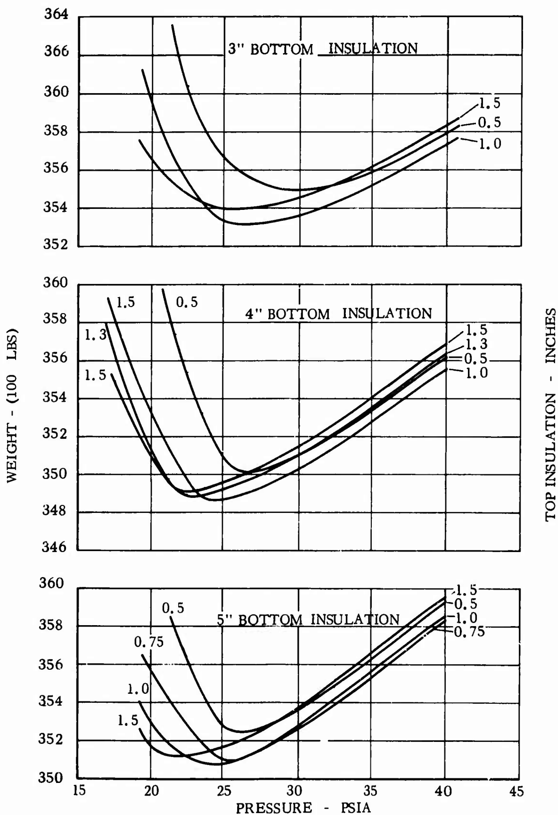
Figure 63. Total Tankage Weight vs. Operating Pressure
