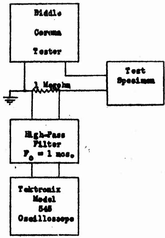
Test Setup for The Measurement of Leakage and Corona Current.
