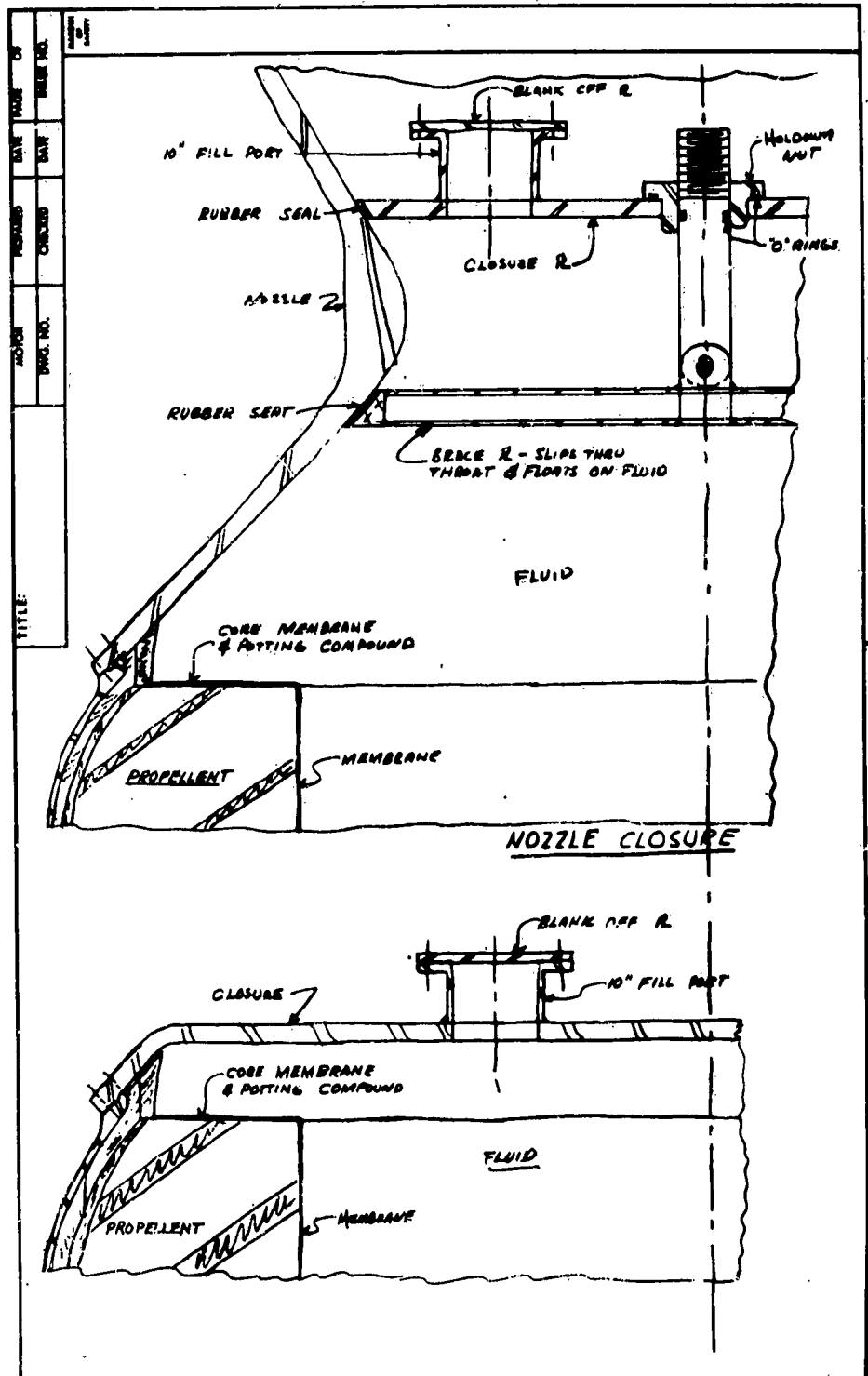
Figure 12. Membrane Core - Case Closure
