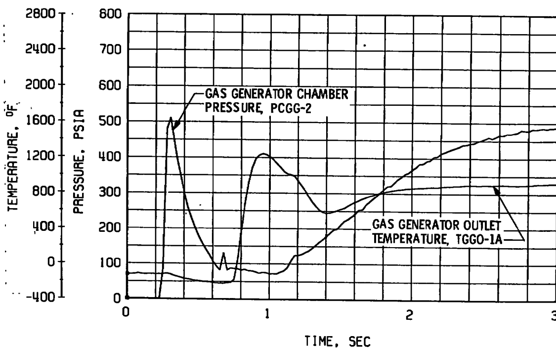
d. Gas Generator Chamber Pressure and Temperature, Start
