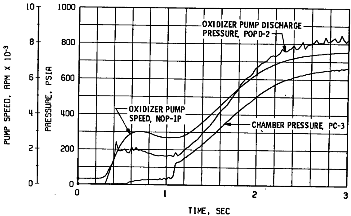
b. Thrust Chamber Oxidizer System, Start Fig. 53 Engine Transient Operation, Firing 27A
