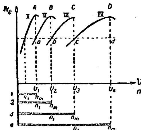
Figure 30. Graphic Illustration of Shifting Levels with Geometric Gradation of the Gears
