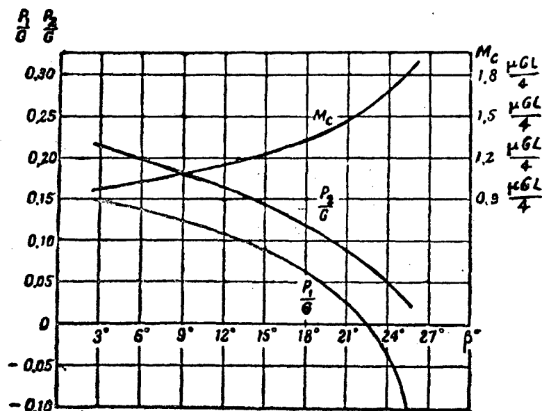
Figure 17. Relation between the moment M_c and the tractive efforts P_2 and P_1 on the one hand, and the angle of bank (angle of inclination \beta ) on the other hand.
