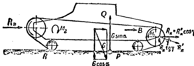
Figure 3. Exterior Forces and Moments of Force effecting the Tank
