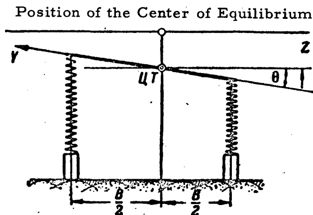
Figure 26. Transverse Vibrations of the Tank Hull
