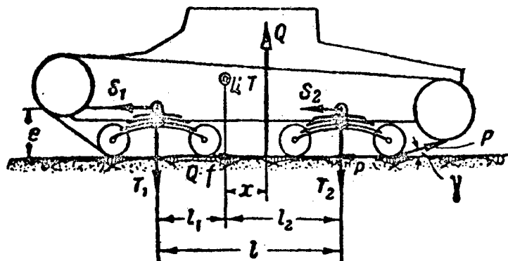
Figure 19. Forces Exerted on the Bogie Wheel Suspension Frame
