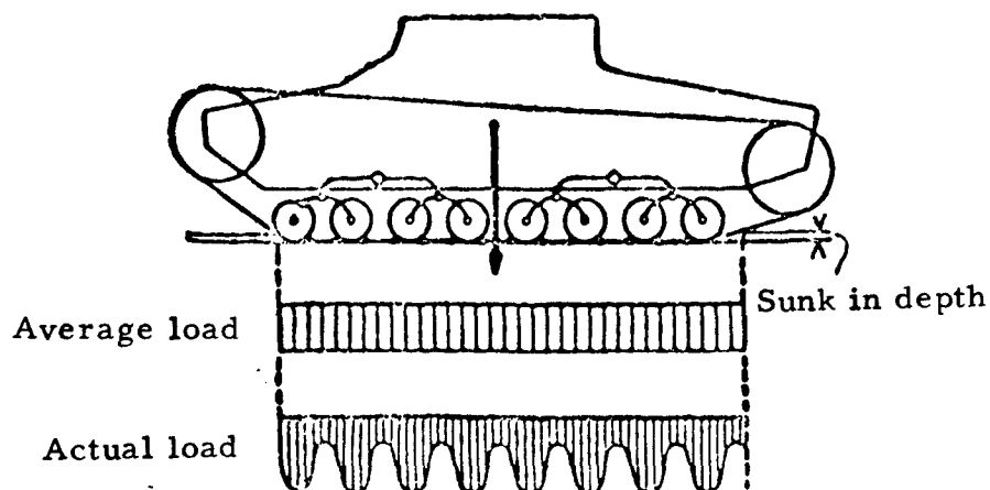
Figure 21. Specific Pressure on Soft Ground
