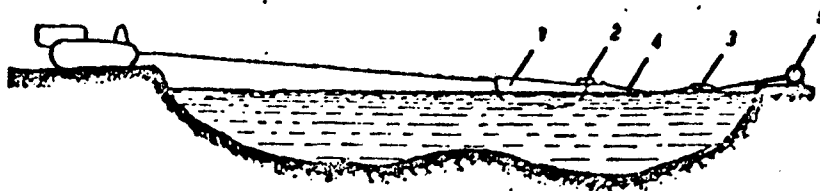
Figure 26. Towing Test with Drive from Land
