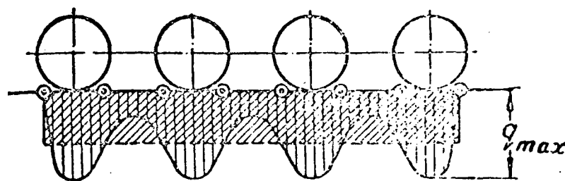
Figure 22. Actual Specific Load on Soft Ground
