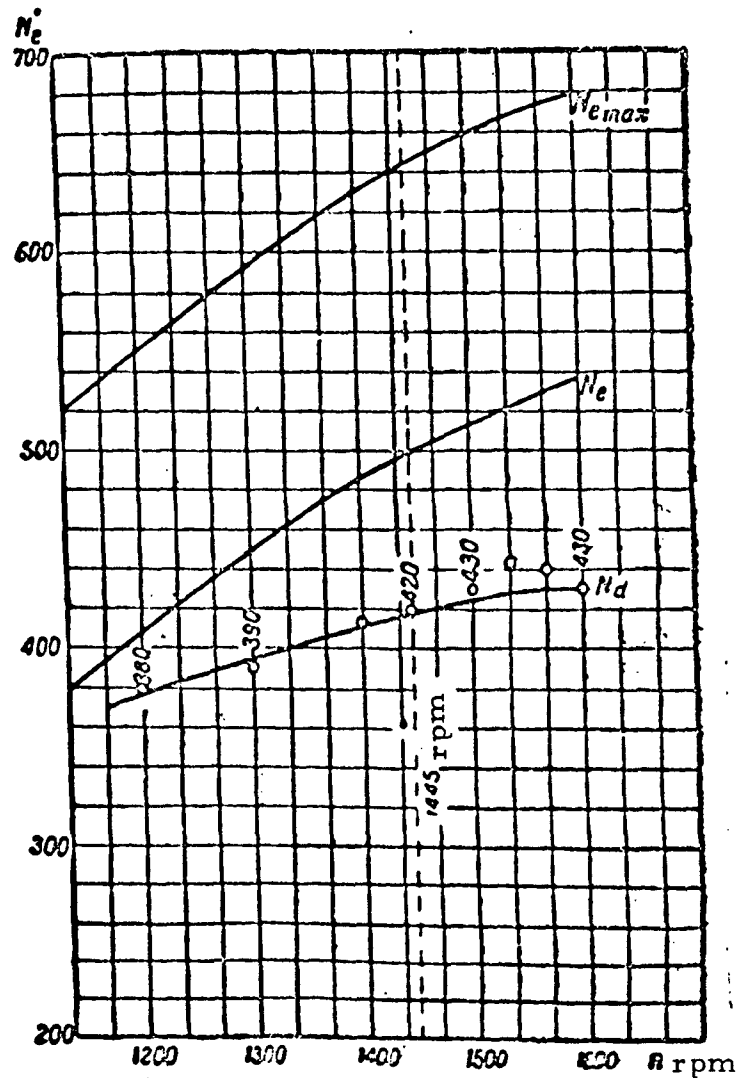
Figure 7. Engine Characteristic Lines with Consideration of Power Loss
