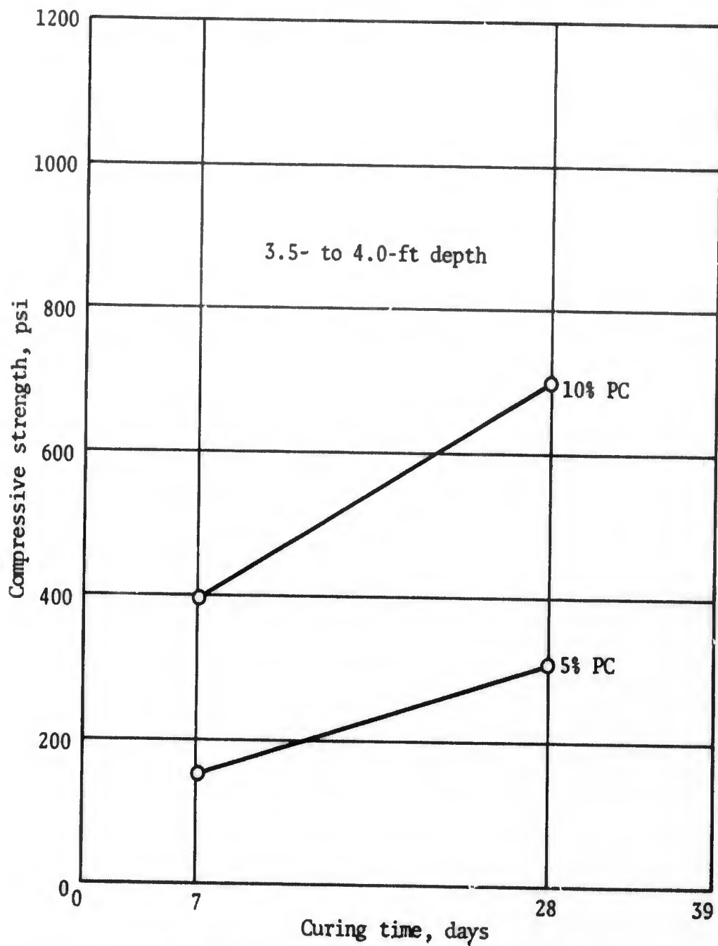
Figure 47. Compressive-strength changes with time in compacted soil-cement mixtures (portland cement), Phan Rang sample 3
