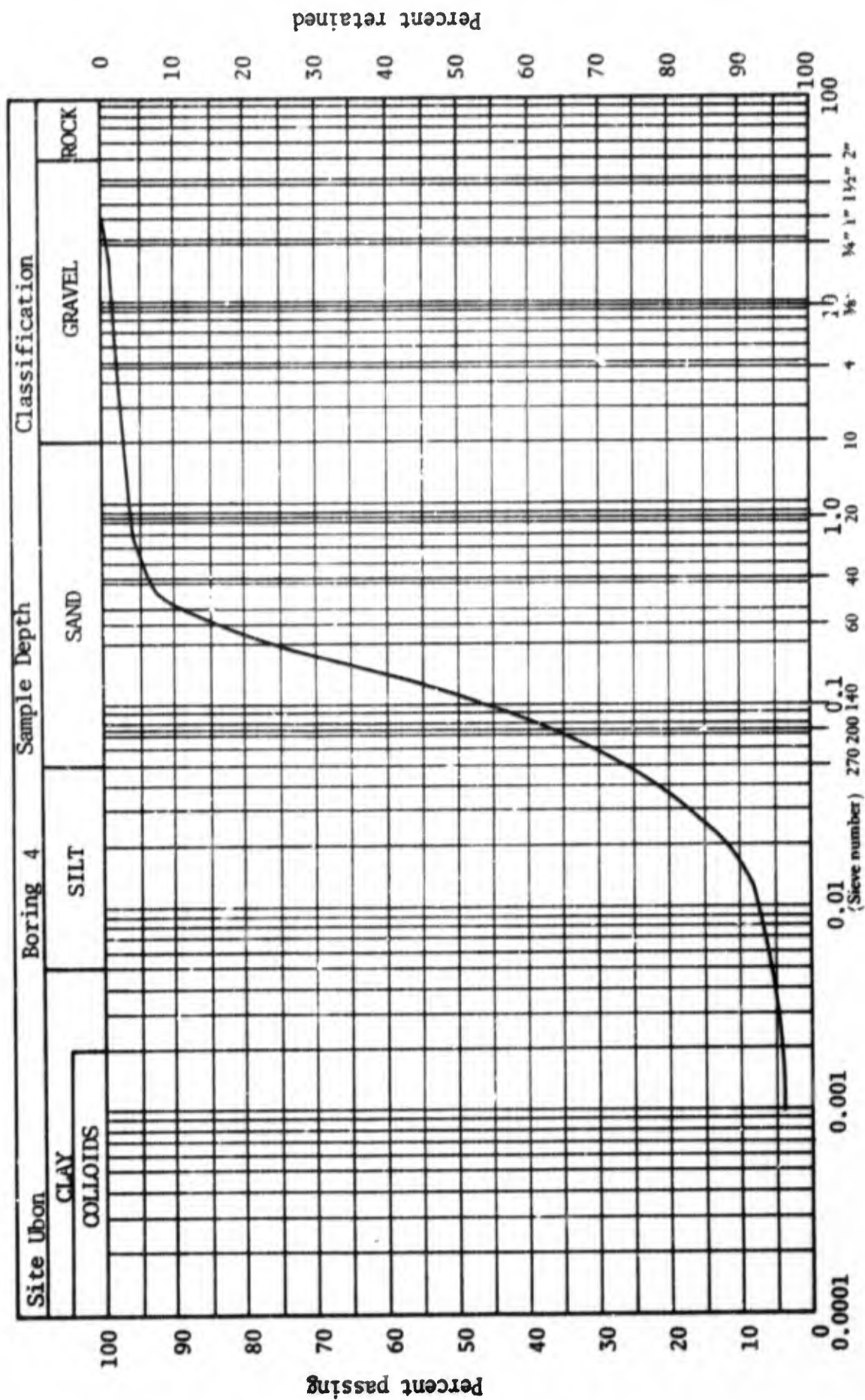
Particle diameter, mm Figure 66. Grain-size distribution curve, Ubon sample 4
