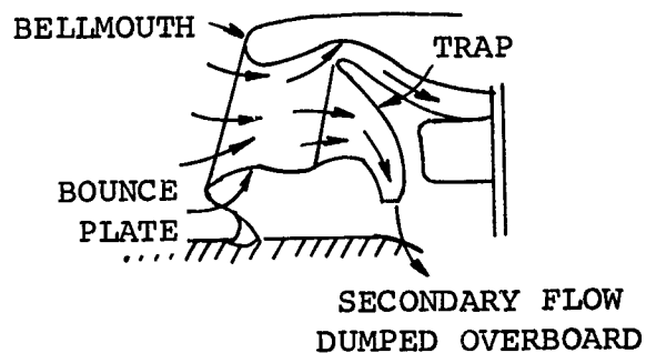
SCHEME 2 BOEING INERTIAL SEPARATOR
