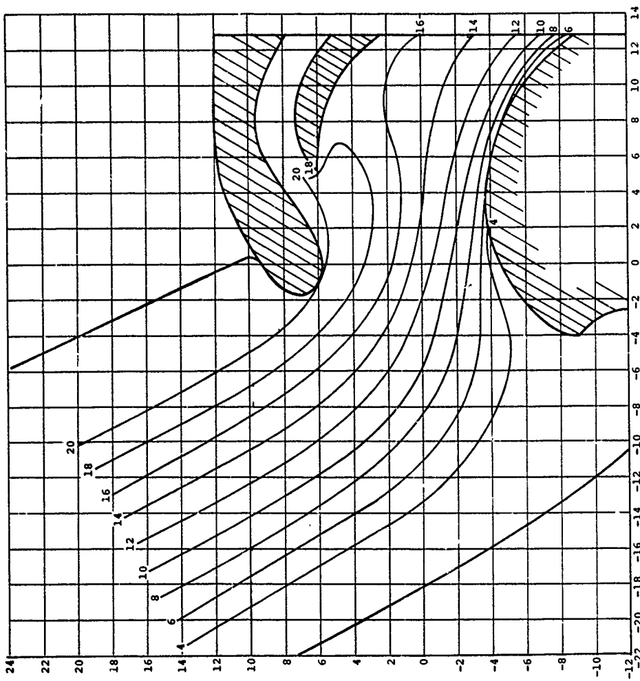
Figure 32. Typical Particle Trajectories
