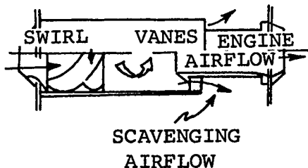
Figure 8. Particle Separator Designs in Current Use
