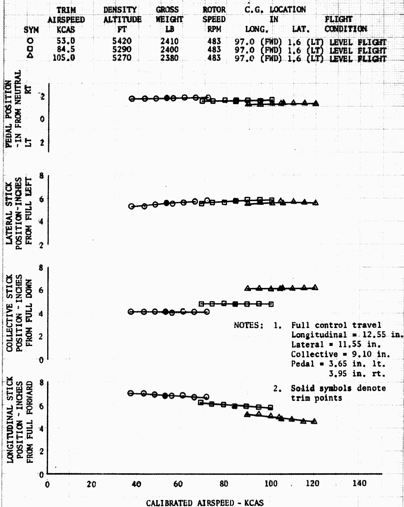
FIGURE NO.14 STATIC LONGITUDINAL COLLECTIVE FIXED STABILITY OH-6A S/N 65-12967 M-27-E1 IN STOWED POSITION
