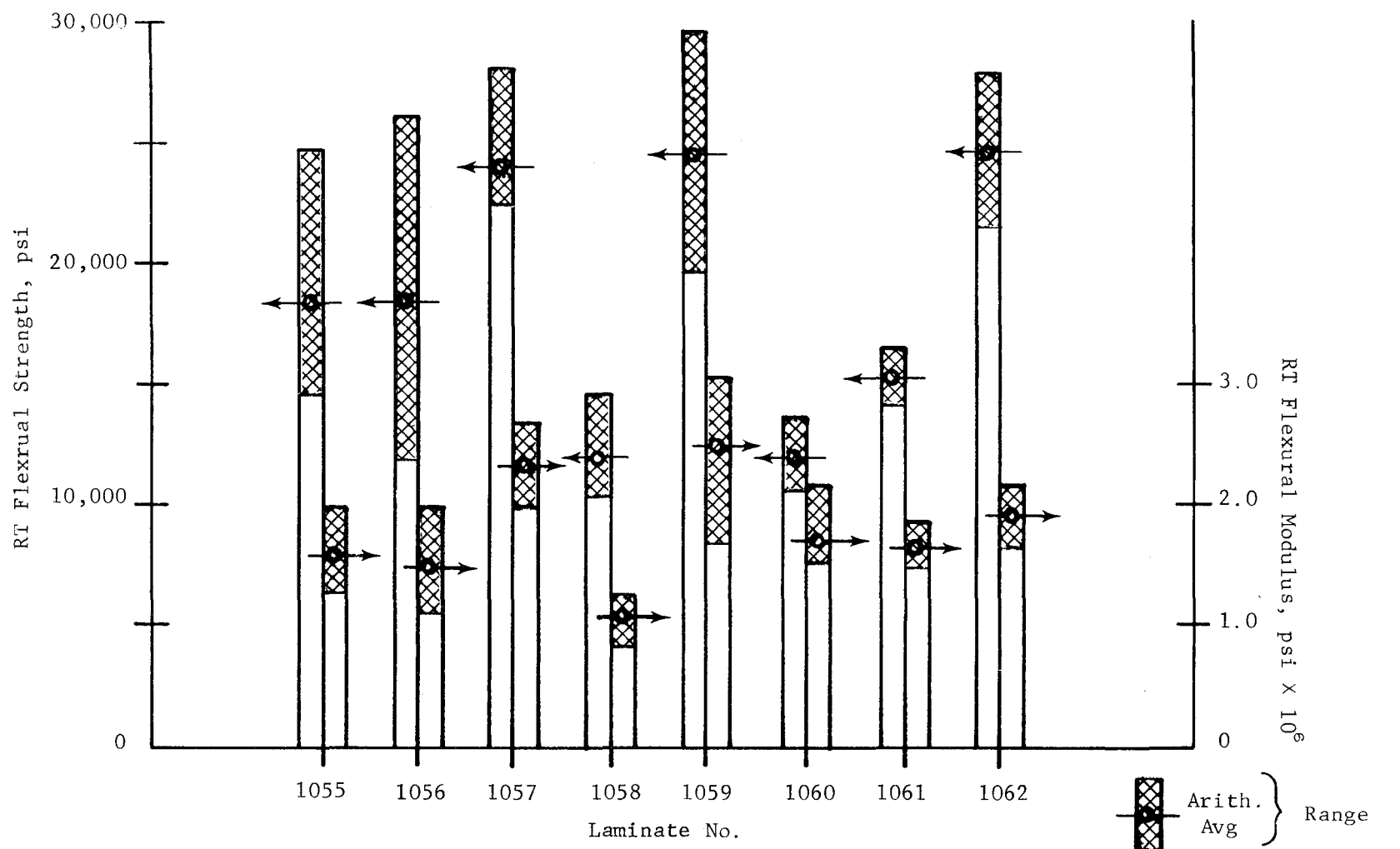
Figure 1. Materials Screening, Selection of Asbestos Reinforcement Material for Skybond 700 Flat Laminates
