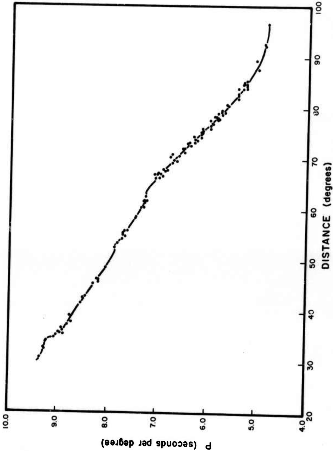
Figure 5. Observed values of p for events with epicenters located along the southeast profile, 140°-160°.
