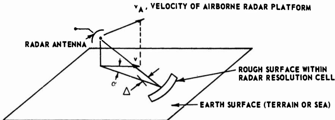
FIGURE 16. GEOMETRY OF SURFACE-DISTRIBUTED CLUTTER VIEWED FROM MOVING RADAR PLATFORM FOR RADAR RESOLUTION CELL OF FINITE DIMENSIONS
