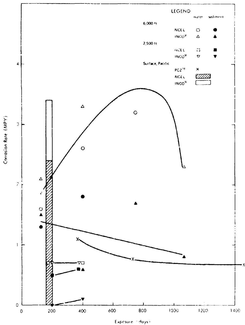
Figure 9 Corrosion rates of Muntz Metal.
