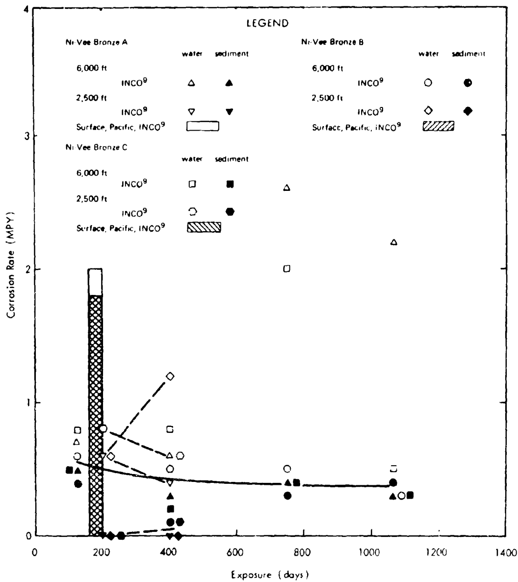
Figure 29. Corrosion rates of Ni - Vee bronzes.
