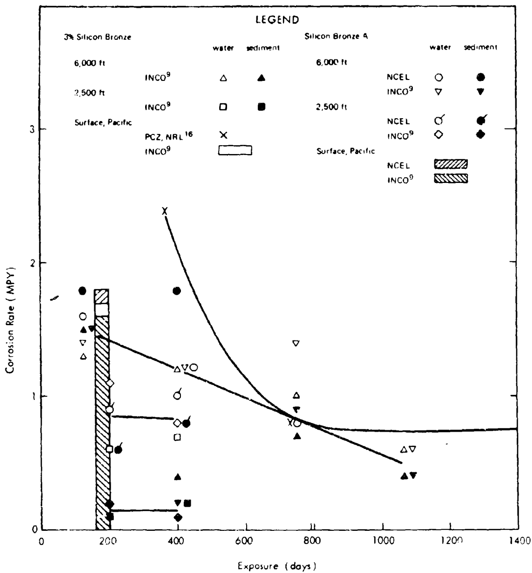
Figure 28. Corrosion rates of silicon bronzes.
