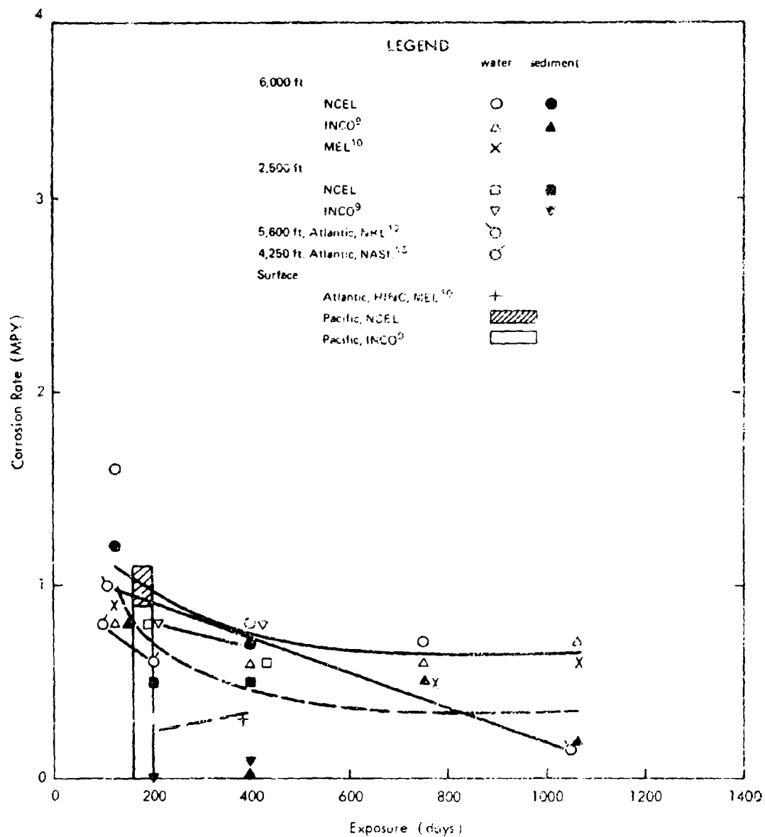
Figure 35. Corrosion rates of 90-10 copper-nickel alloy.
