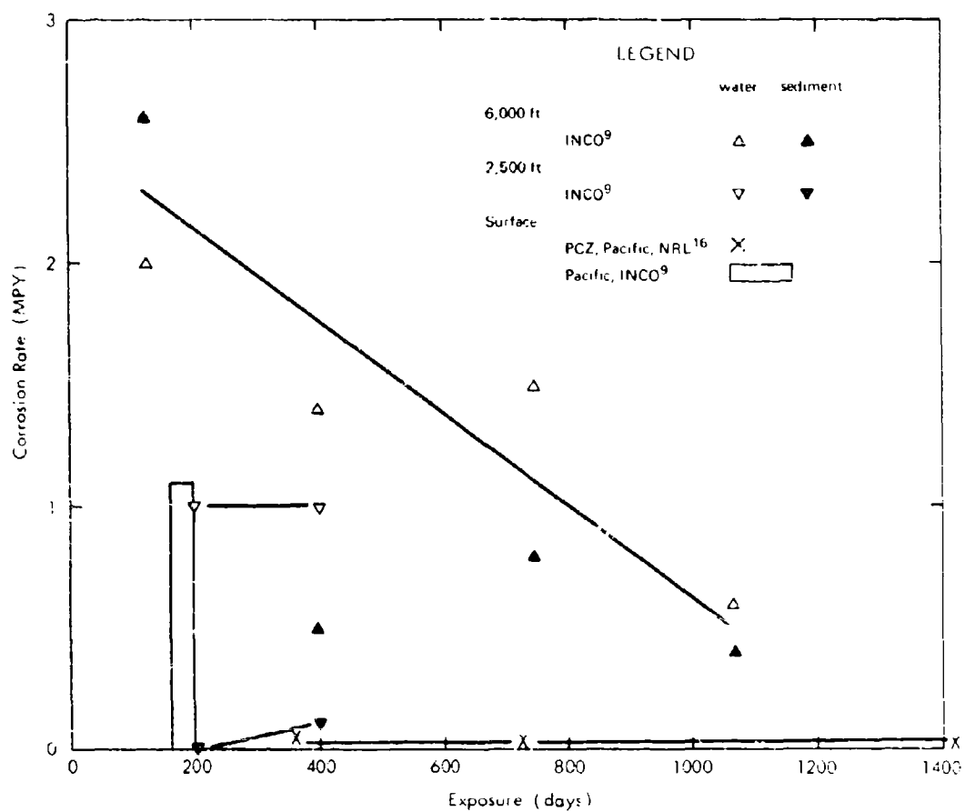
Figure 42. Corrosion rates of 65-18 nickel-silver alloy.
