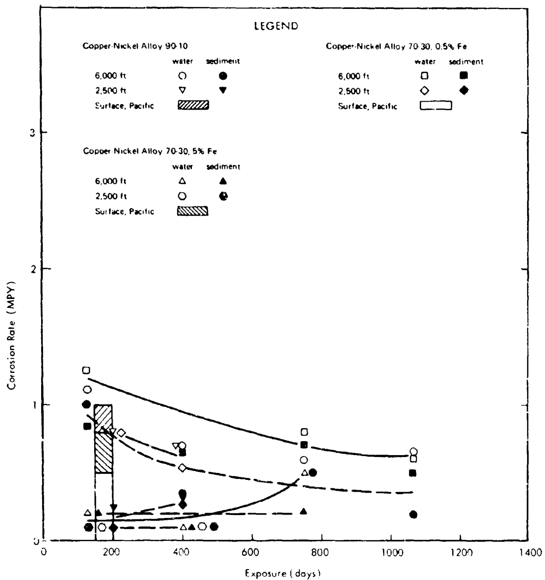
Figure 38. Corrosion rates of copper-nickel alloys.
