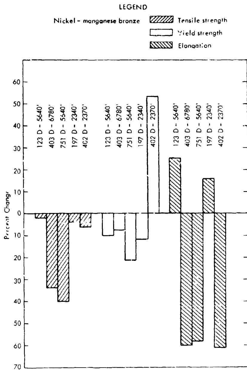
Figure 21. Effects of exposure on mechanical properties of nickel-manganese bronze.
