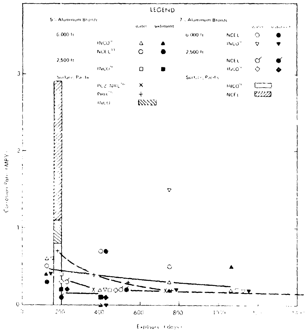
Figure 25. Corrosion rates of wrought aluminum bronze.
