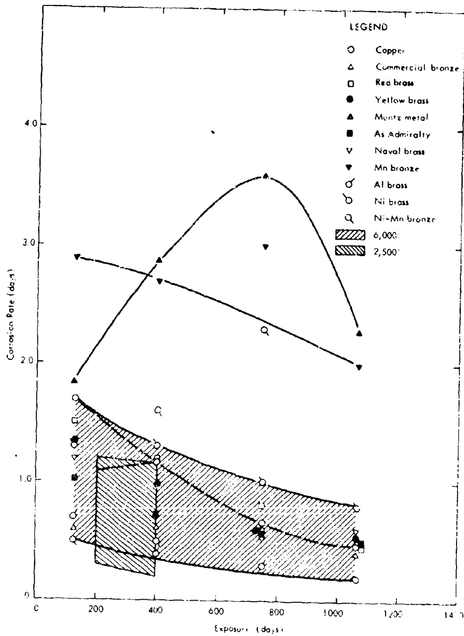
Figure 17. Corrosion rates of copper-zinc alloys in sea water.
