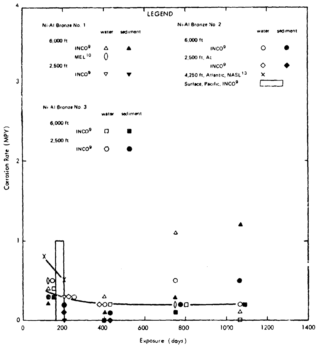
Figure 27. Corrosion rates of nickel - aluminum bronzes.
