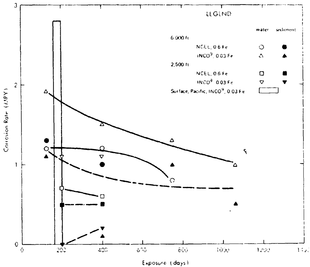
Figure 40. Corrosion rates of 80-20 copper-nickel alloy.
