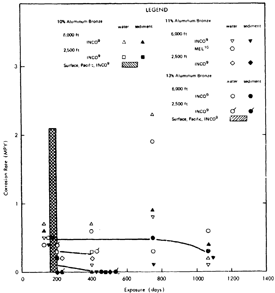
Figure 26. Corrosion rates of cast aluminum bronzes.
