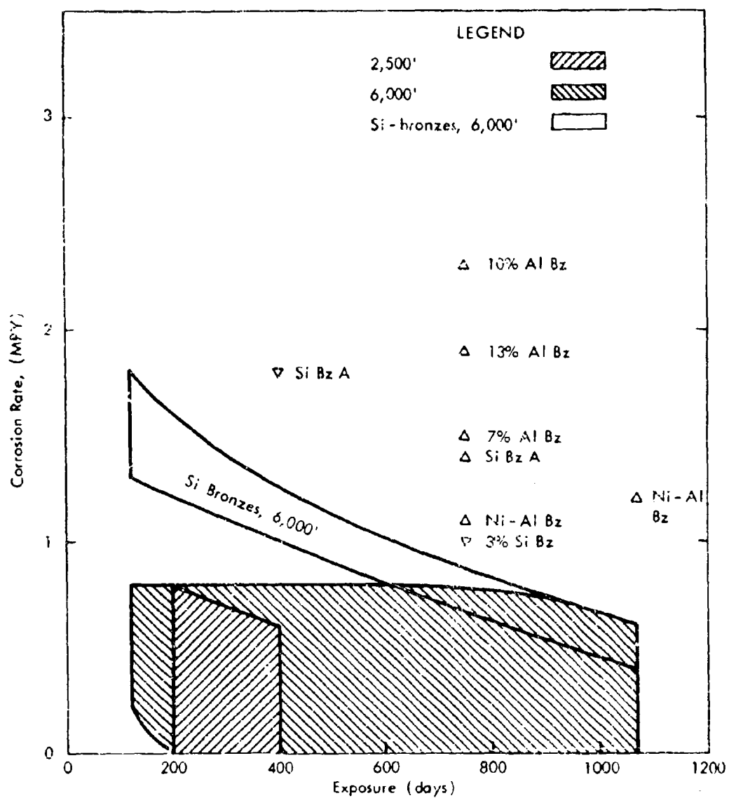
Figure 30. Corrosion rates of bronzes.
