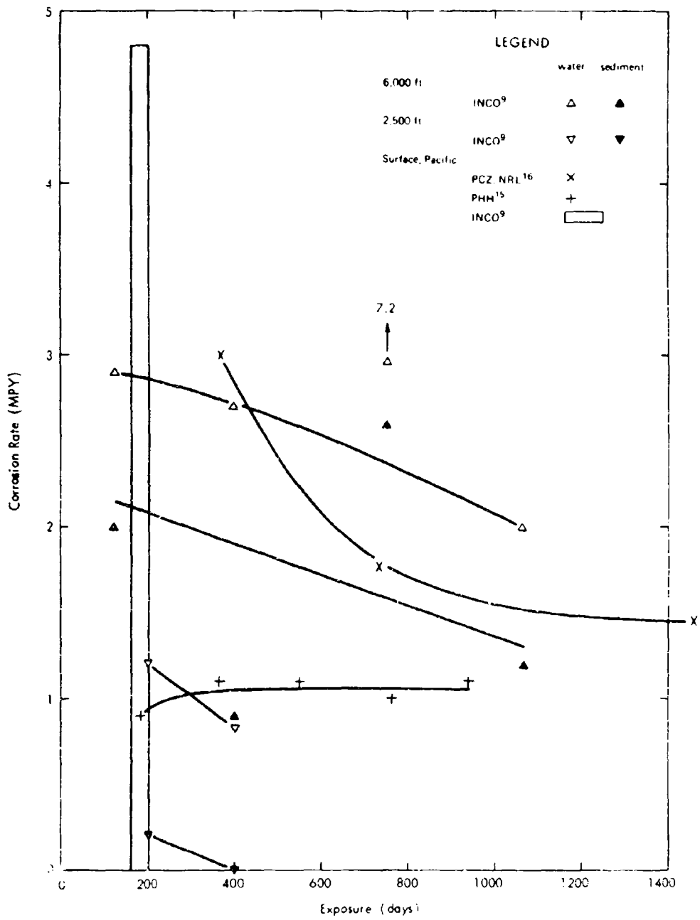
Figure 12. Corrosion rates of manganese bronze.
