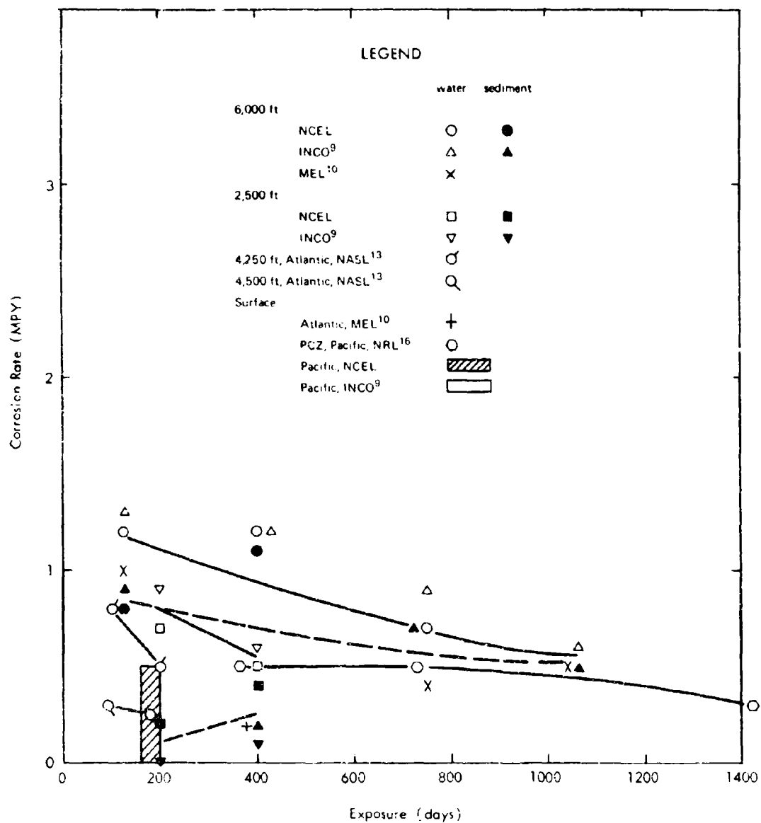
Figure 36. Corrosion rates of 70-30 copper-nickel alloy containing 0.5 % iron.
