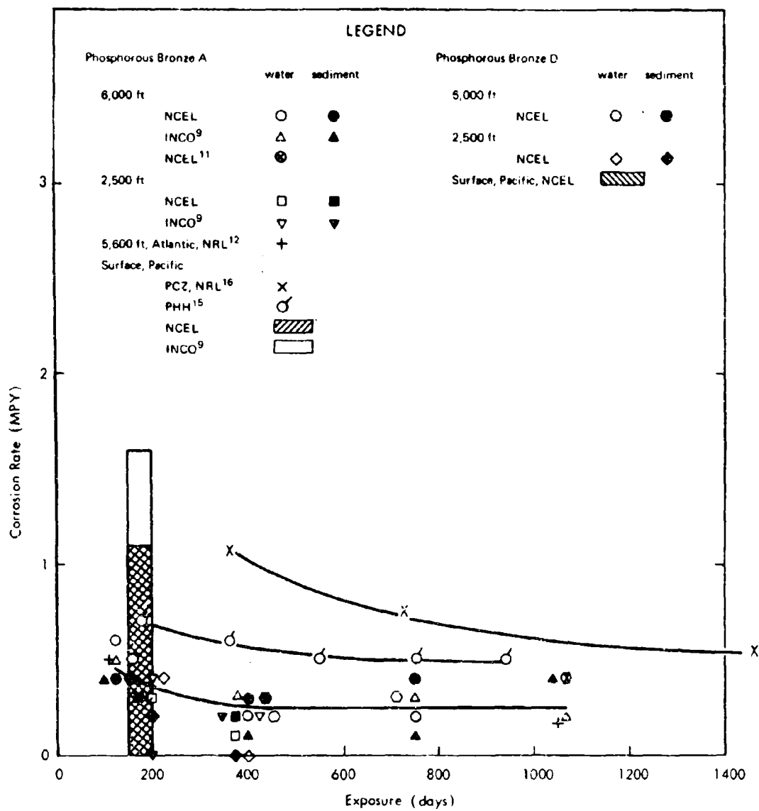
Figure 24. Corrosion rates of phosphorous bronzes A and D.
