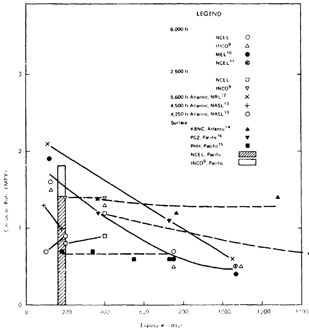
Figure 3. Corrosion rates of copper in sea water.
