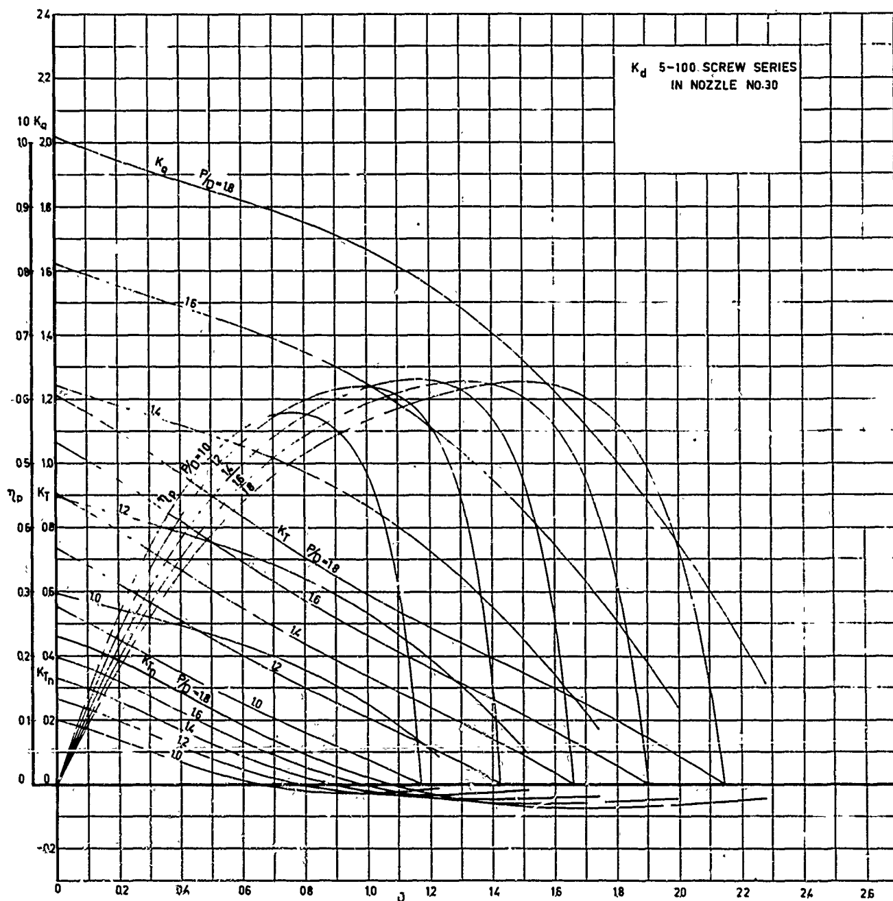
Fig.18 Open water test results of nozzle no.30 ( K_t , K_p , K_d and \eta_p as functions of J ).
