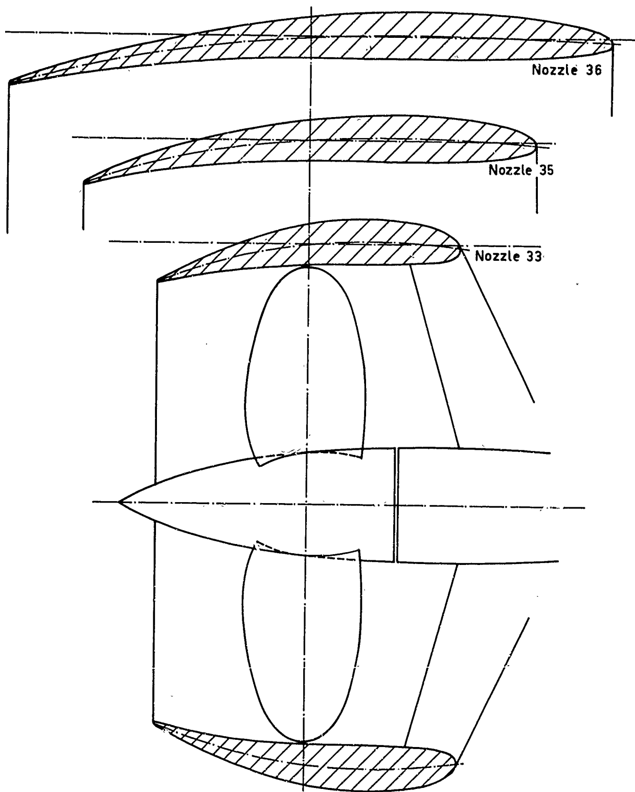
Fig.14 Particulars of nozzles nos. 33, 35 and 36.
