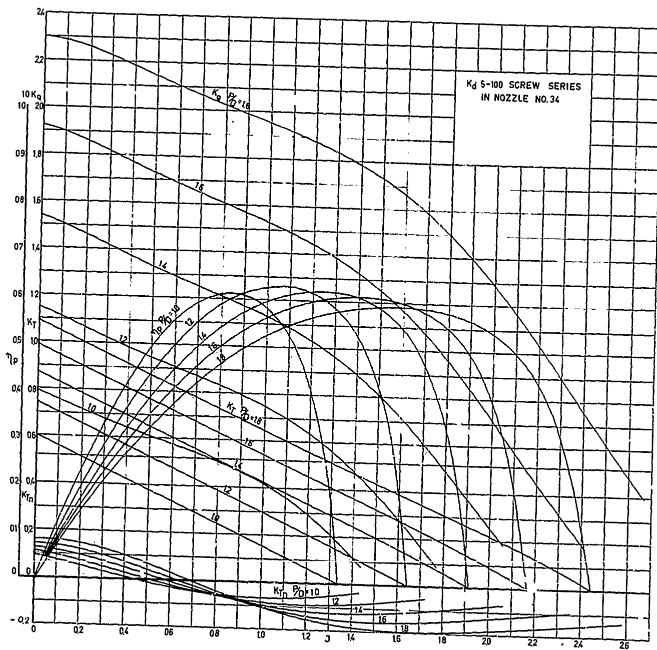
Fig.22 Open water test results of nozzle no.34 ( K_T ; K_{Tn} ; K_Q and \eta_p as functions of J ).
