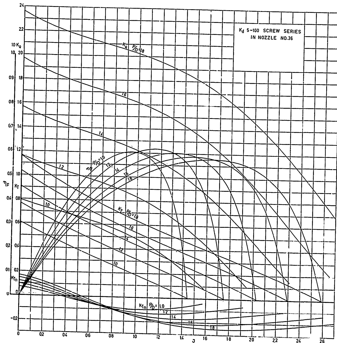
Fig.24 Open water test results of nozzle no.36 ( K_T , K_{Tn} , K_Q and \eta_p as functions of J )
