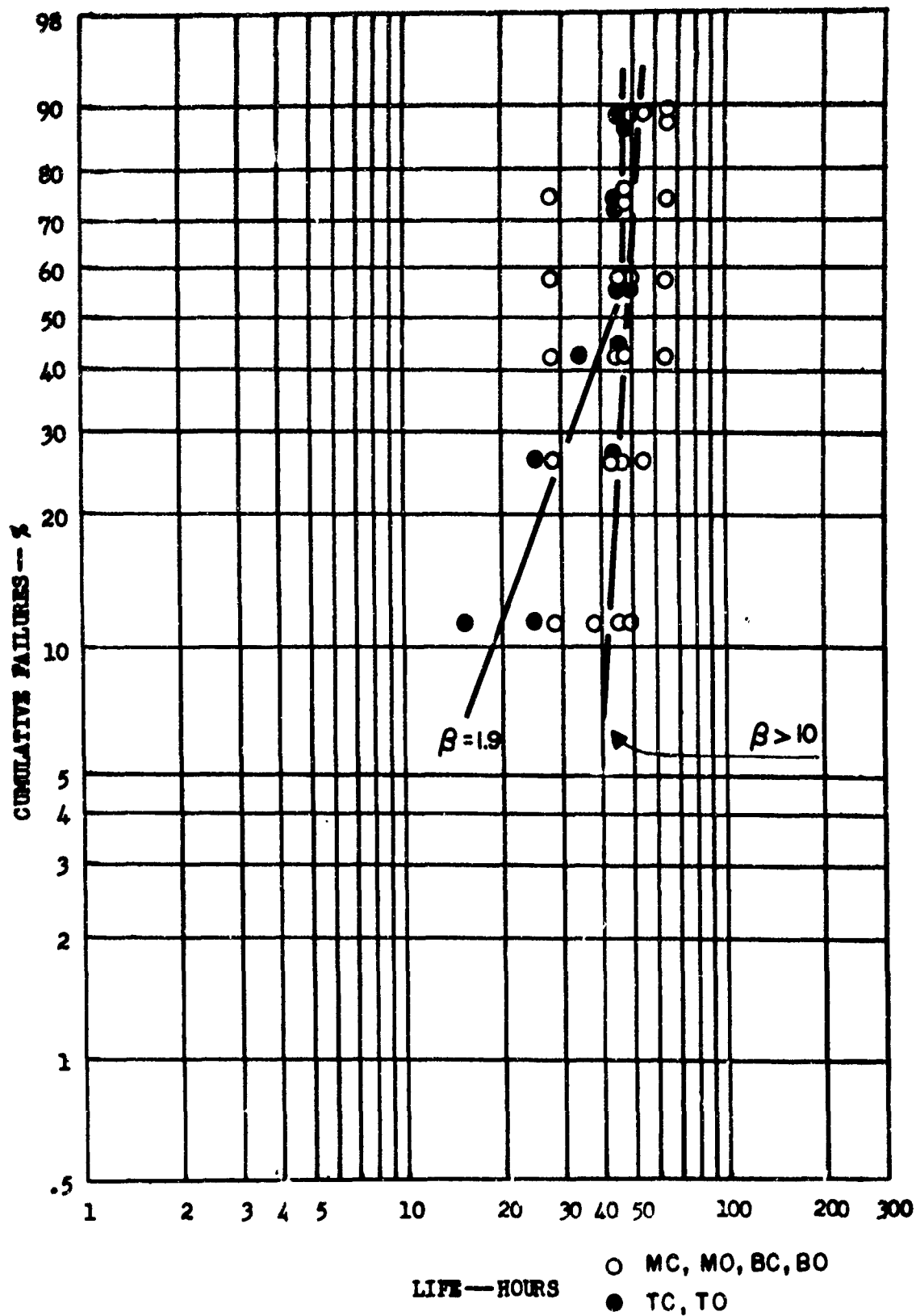
Percent Cumulative Failure Versus Cyclic Oxidation Life at 2700°F for Specimens Coated in Module Run #4, Pack Position Breakout.
