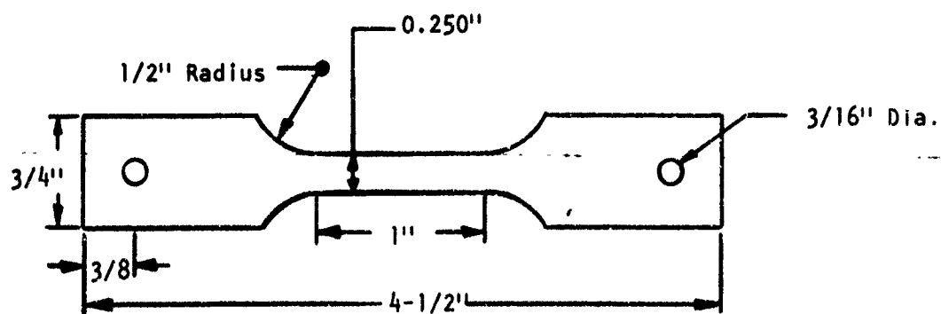
TENSILE TEST SPECIMEN
