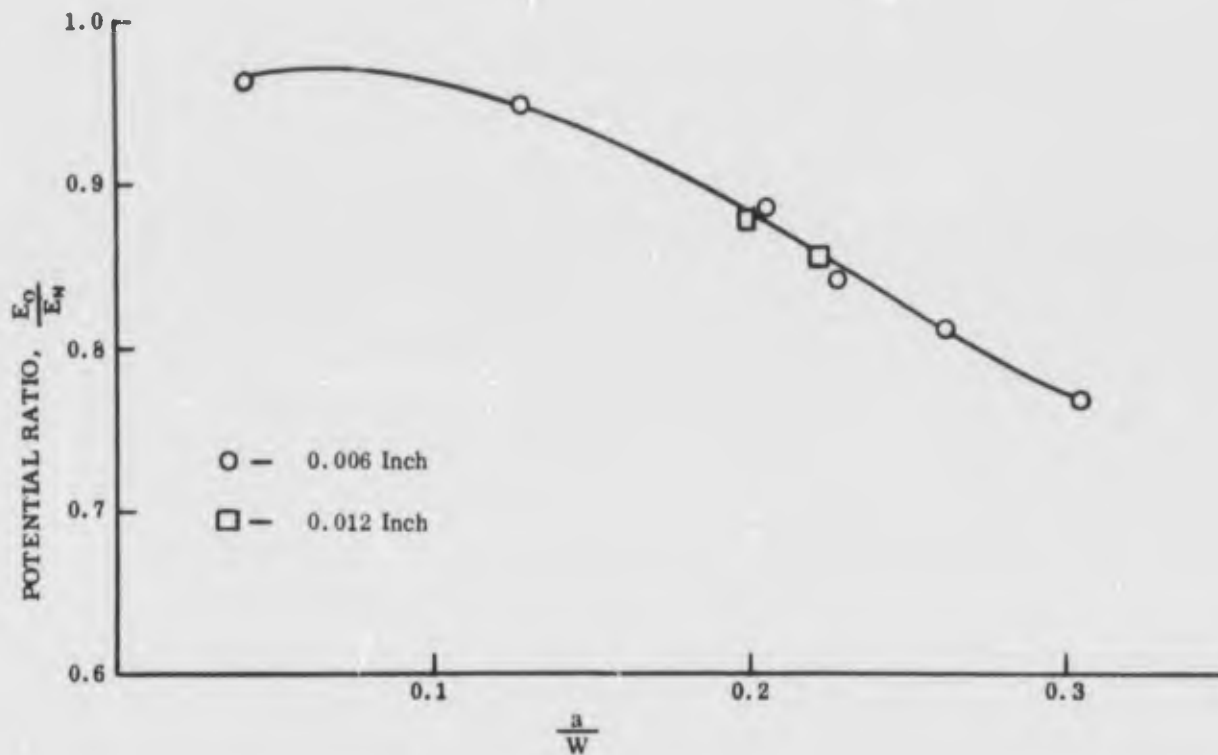
FIGURE 26. CALIBRATION CURVE RELATING ELECTRICAL POTENTIAL AND NOTCH LENGTH FOR CENTER NOTCHED TZM SPECIMENS
