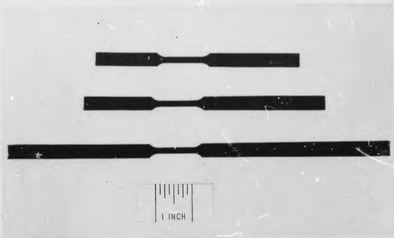
FIGURE 41. TITANIUM-BORON TAPES AFTER DIFFUSION BONDING AND TRIMMING
