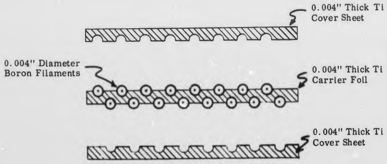
FIGURE 39. COMPONENTS OF A Ti-B COMPOSITE TAPE
