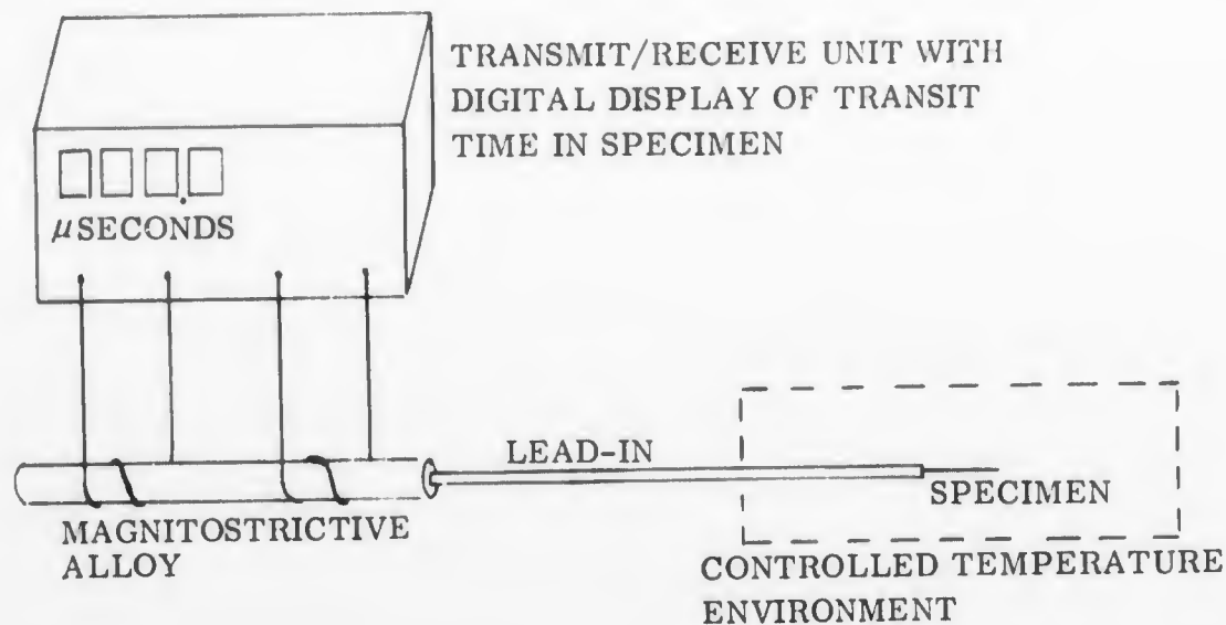
FIGURE 19. SCHEMATIC OF ULTRASONIC METHOD USED BY PARAMETERS TO MEASURE MODULI OF THIN-GAGE TD NICKEL ALLOY
