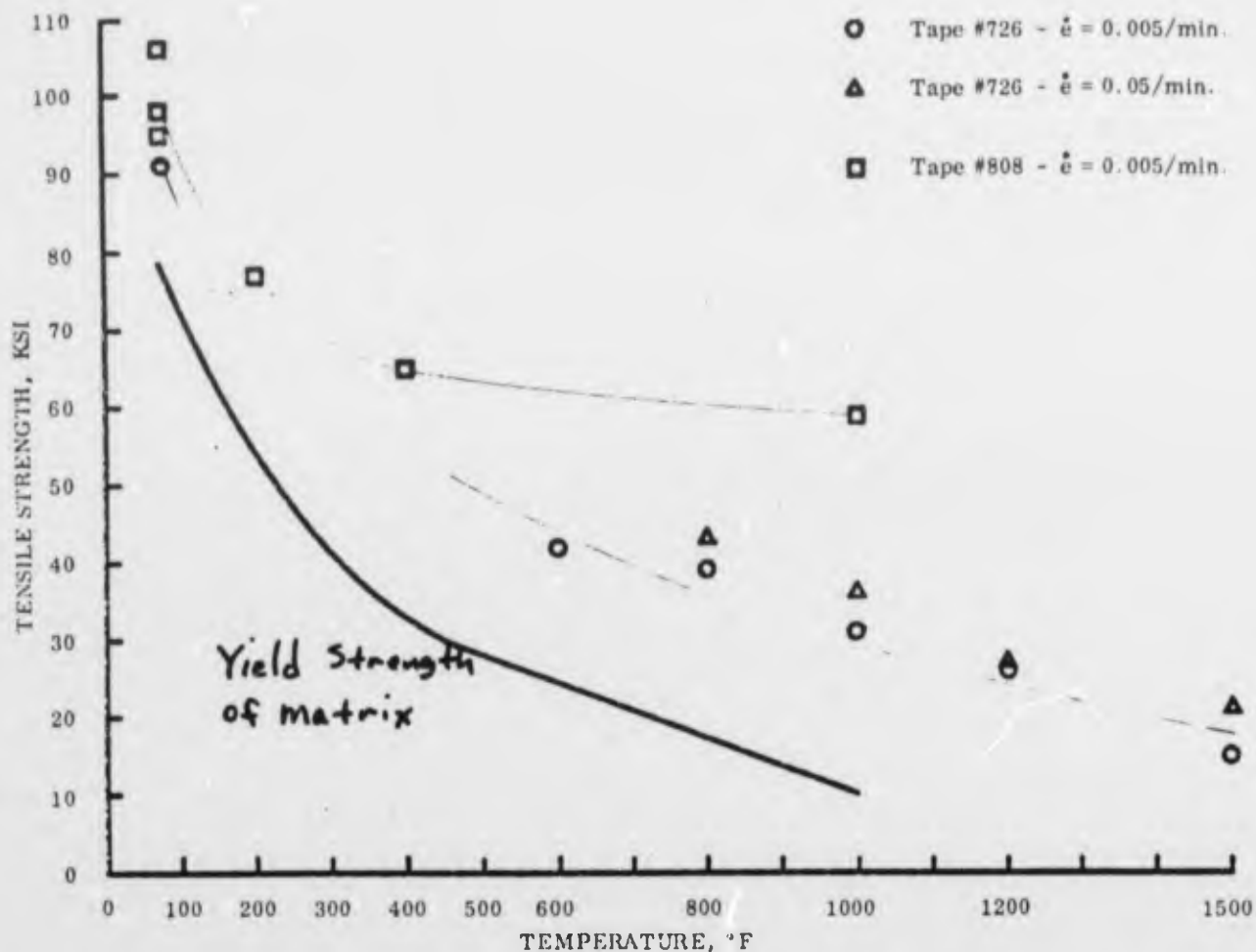
FIGURE 44. TENSILE STRENGTH VERSUS TEMPERATURE FOR Ti-B COMPOSITE TAPES (23 Volume Percent B in Ti-75A Matrix)
