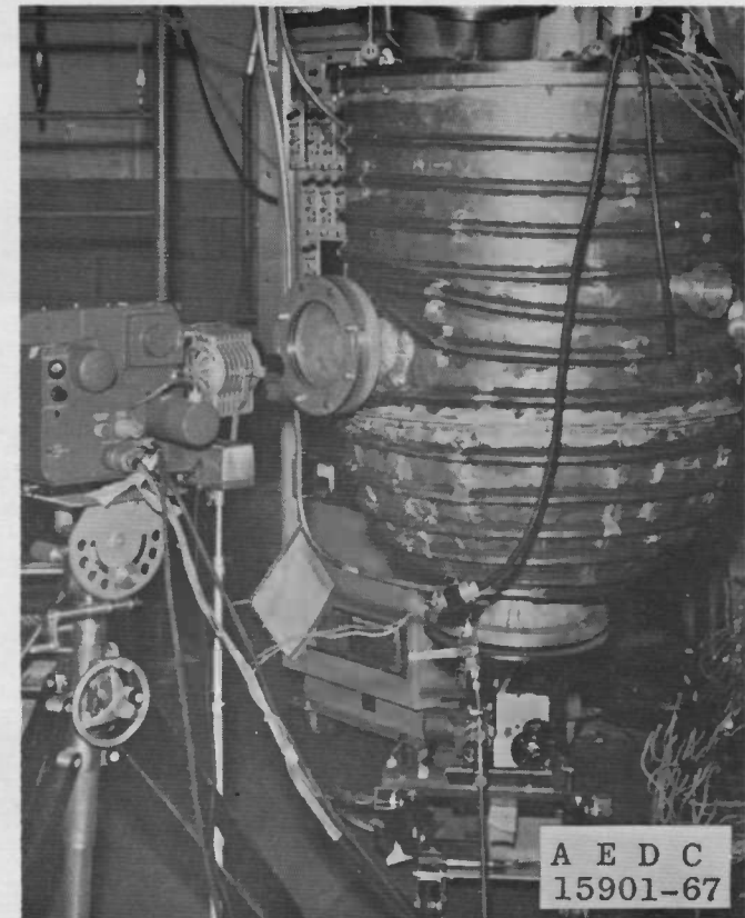
Fig. 8 Modified Antechamber after Installation - Ready for ARC (8V) Tests
