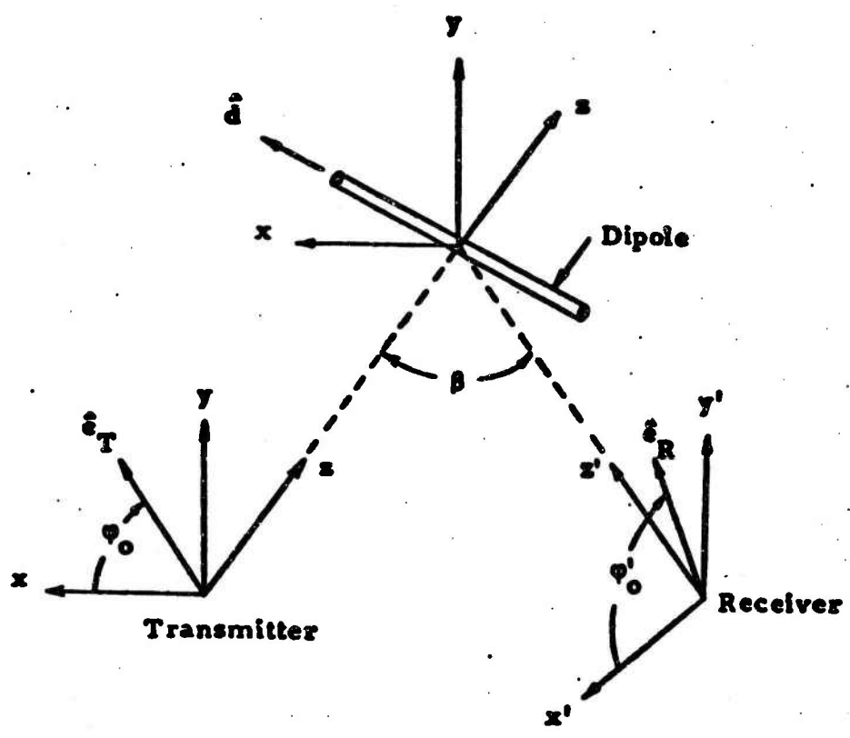
Fig. 1 - Bistatic Scattering Geometry
