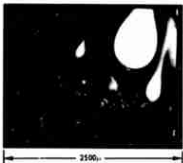
FIG. 3.3 Selected frames from high speed motion picture of composite propellant containing 18% aluminum burning at 100 psi.
