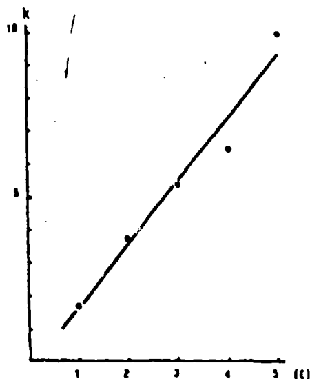
Figure 2. Variation of the first order constant in the last portion of the emission curves as a function of the enzyme concentration. Concentration of reactants: Lymnoxanthine 10^{-4} M., buffer of carbonate-bicarbonate pH 9.7, concentration 2.5 \times 10^{-2} M. (E): enzyme concentrations \times 1/320 . Values of k in \text{min.}^{-1} . Temperature 17^\circ\text{C} .
