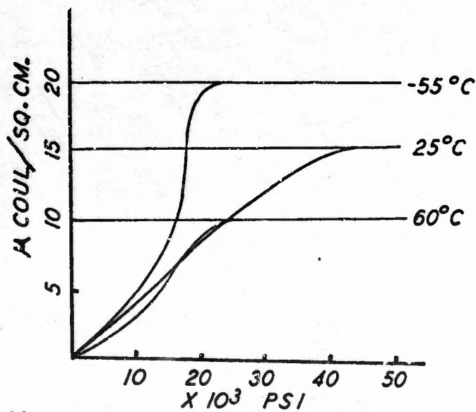
FIG. 11 CHARGE OUTPUT VERSUS HYDROSTATIC LOADING AS A FUNCTION OF TEMPERATURE FOR X=.2 Y=.04
