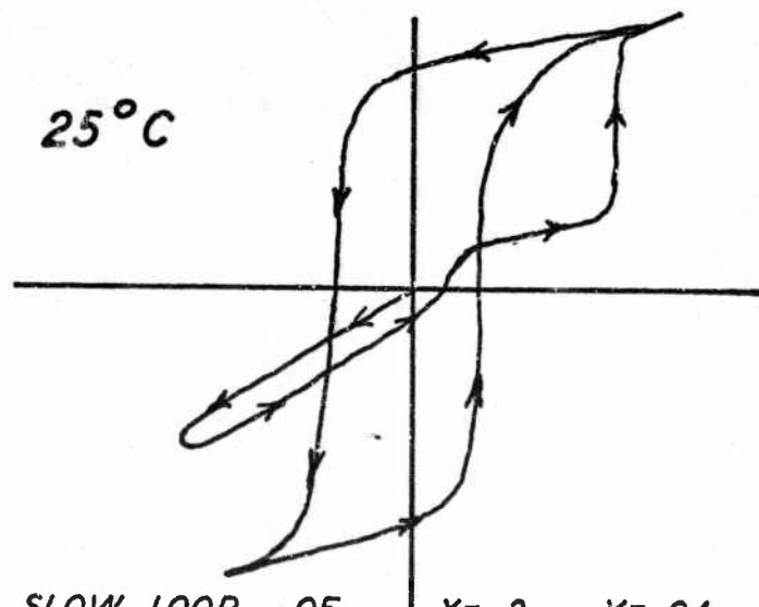
FIG. 13 SLOW LOOP OF X=.2 Y=.04
