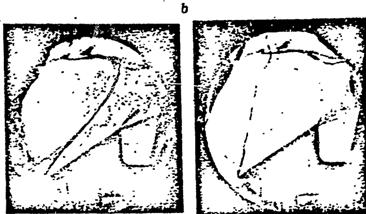
Fig. 17. Arrangement of slanting waves for Ma = 3.0 : a) \bar{Q} = 0 ; b) \bar{Q} = 1.3
