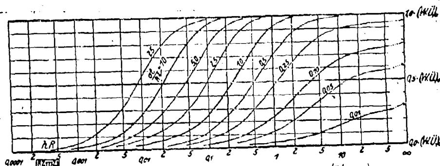
Figure 3. Heat loss of sphere when \Theta_c = 10 ; Q = (W U)_0 \Psi \left( \frac{\alpha t}{R^2}, \lambda R \right) .
