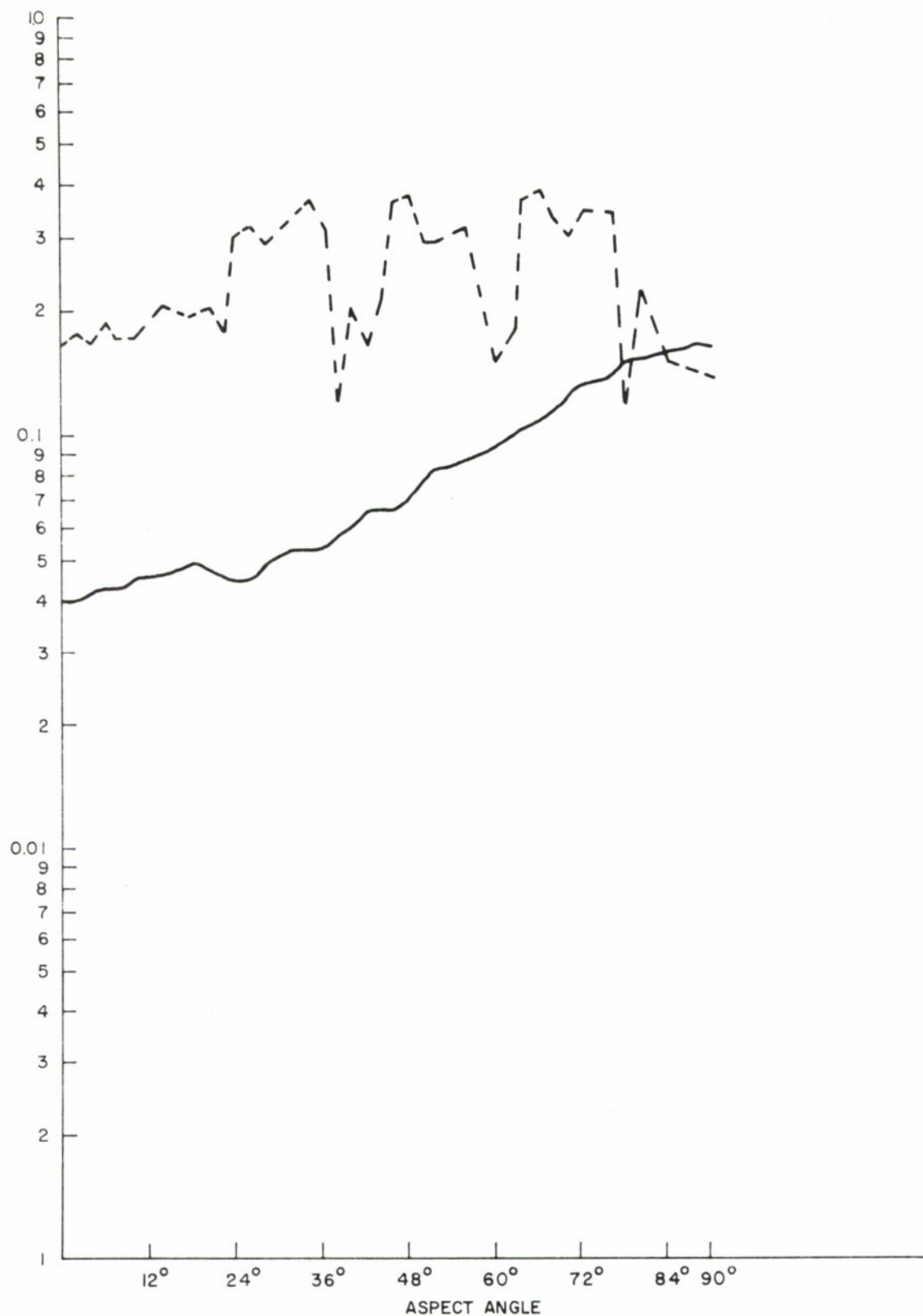
Figure 65. THE S-MATRIX ELEMENT s_{LR} (SOLID) AND D = s_{LL} / s_{LR} (DOTTED) VERSUS ASPECT ANGLE FOR BODY NO. 5 (PHASE ADJUSTED BY -19^\circ )
