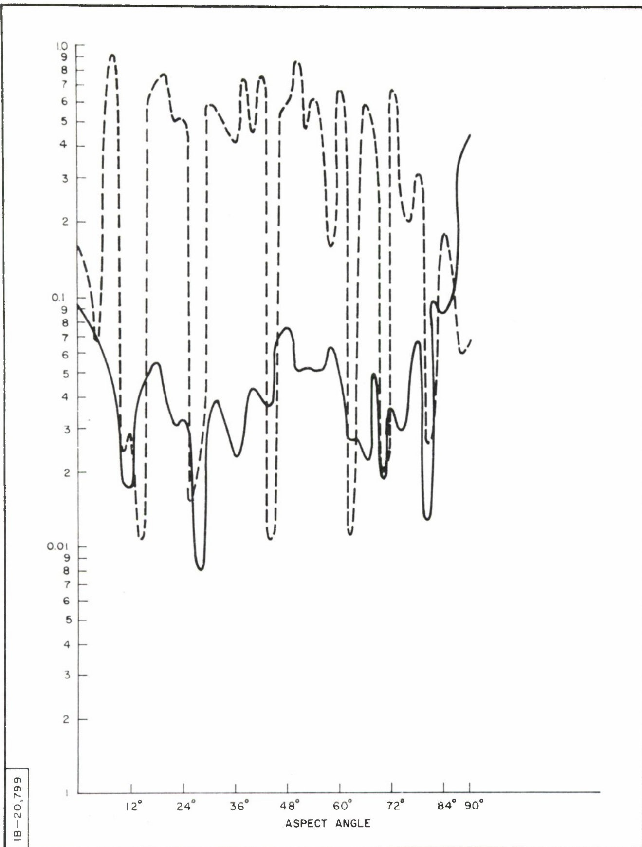
Figure 35. THE S-MATRIX ELEMENT s_{LR} (SOLID) AND D = s_{LL} / s_{LR} (DOTTED) VERSUS ASPECT ANGLE FOR BODY NO. 8
