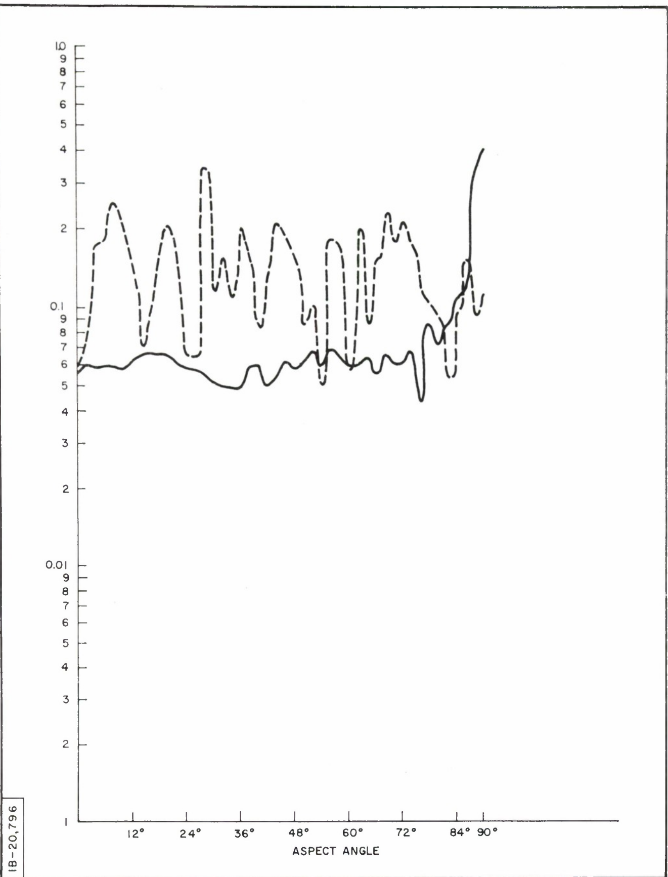
Figure 43. THE S-MATRIX ELEMENT s_{LR} (SOLID) AND D = s_{LL}/s_{LR} (DOTTED) VERSUS ASPECT ANGLE FOR BODY NO. 16
