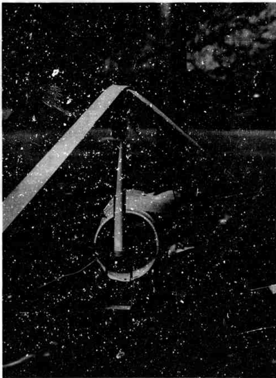
Figure 7. Typical Test Setup A. Rate Stick C. Plexiglas Column B. Shield Plate D. Argon Bomb
