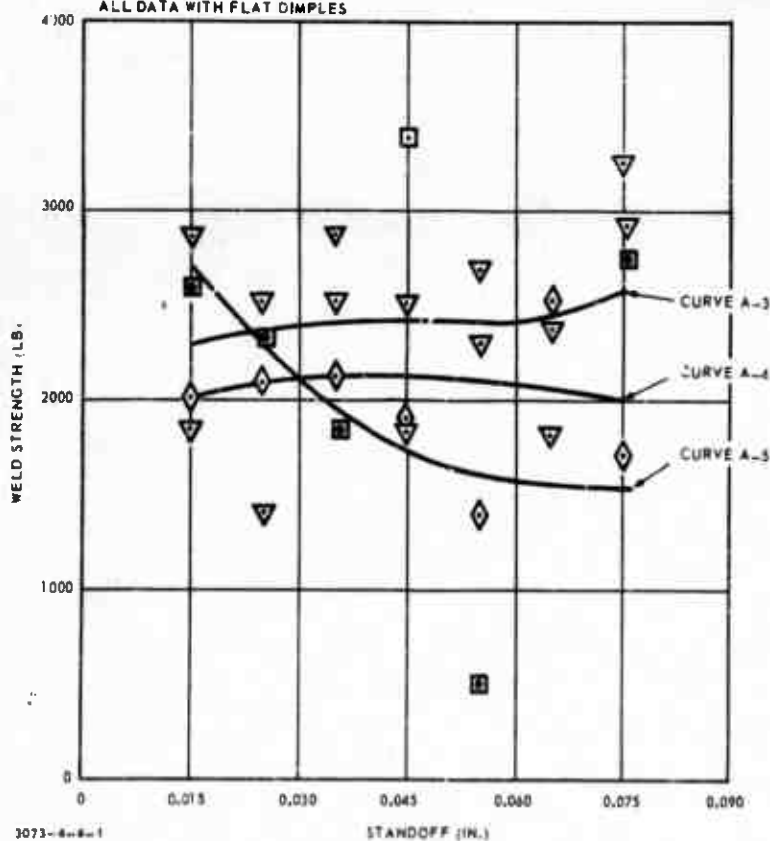
Figure 22. Weld Strength vs Standoff for Type 347 Stainless Steel 0.063 in. Thick. (b)
