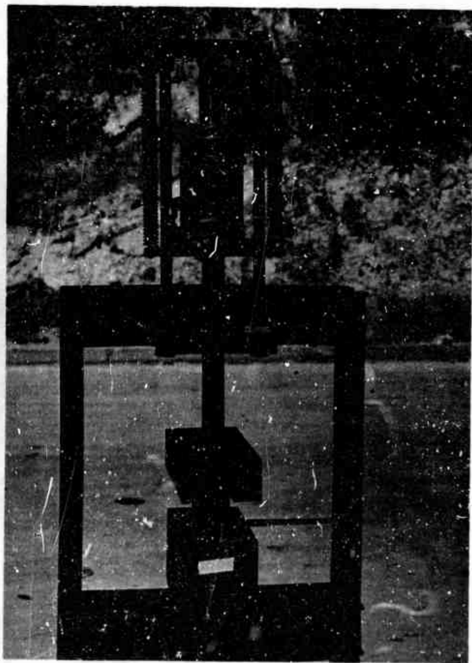
Figure 3. Press Operated Tooling for Explosive Spot Welding.
