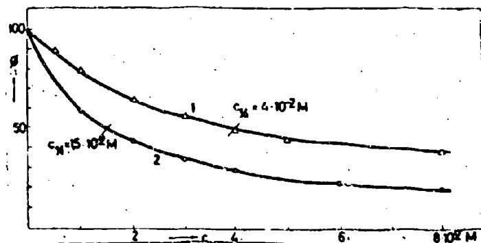
Figure 1. Quenching of the fluorescence of luminol in solutions by the oxime of pyrroacetic acid (1) and by pyridine-4-aldoxime (2). \phi - intensity of the fluorescence, c - concentration of the oxime.
