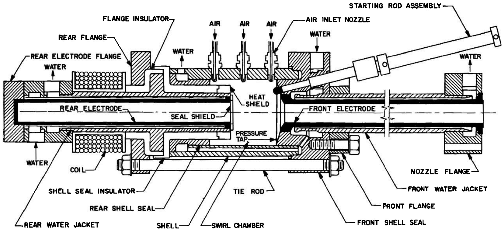
Fig. 3 Schematic of Modified Linde N-4000 Arc Heater
