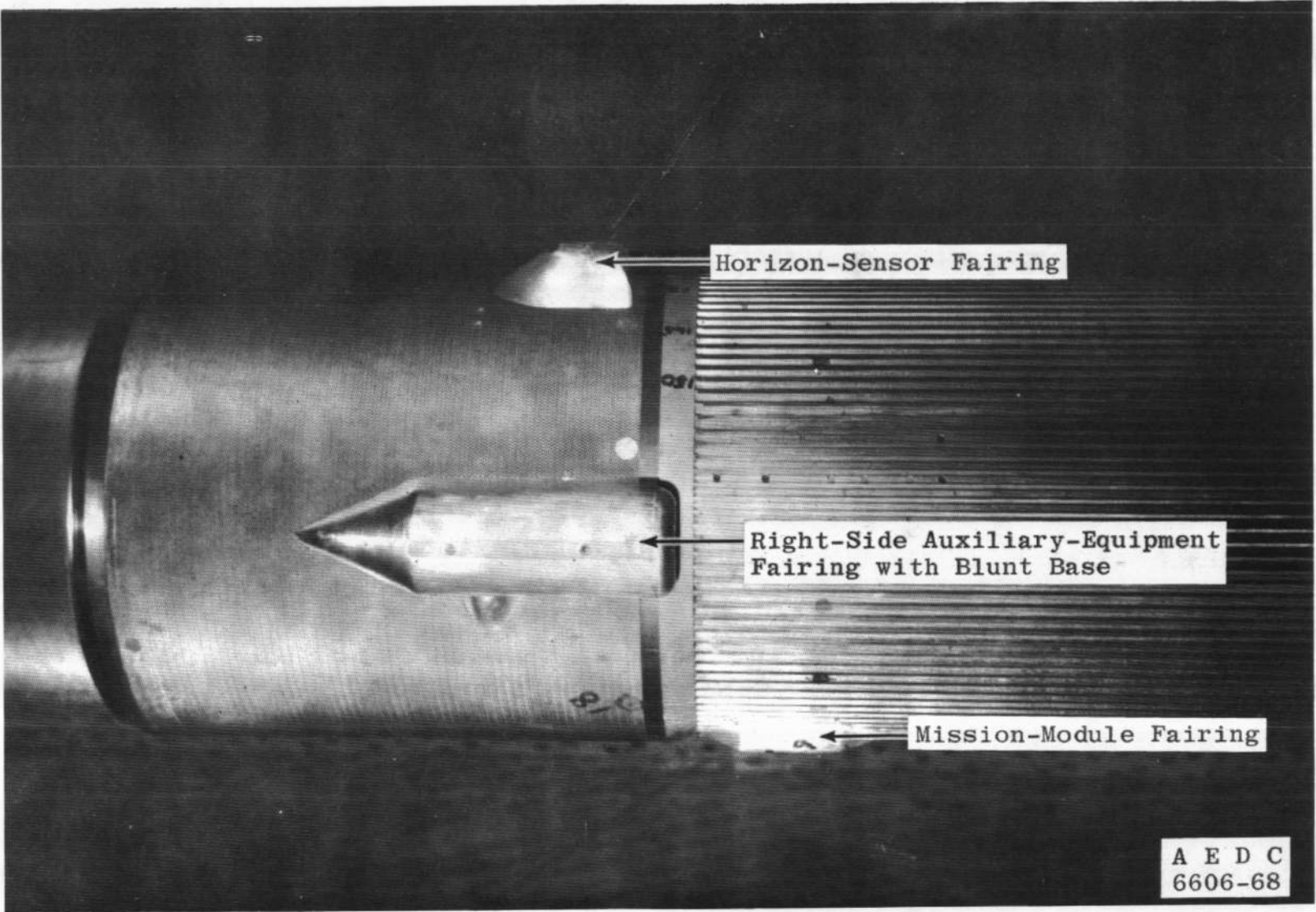
b. Configuration 1, Blunt Base on Right-Side Auxiliary-Equipment Fairing Fig. 5 Continued
