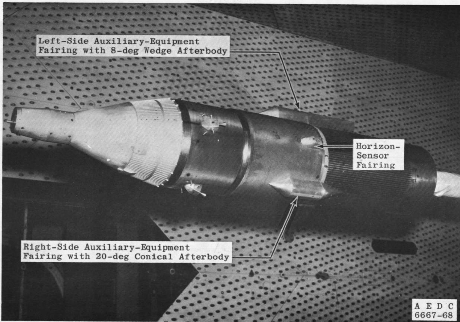
c. Configuration 2, 20-deg Cone and 8-deg Wedge Afterbody on Right- and Left- Side Auxiliary-Equipment Fairing, Respectively
