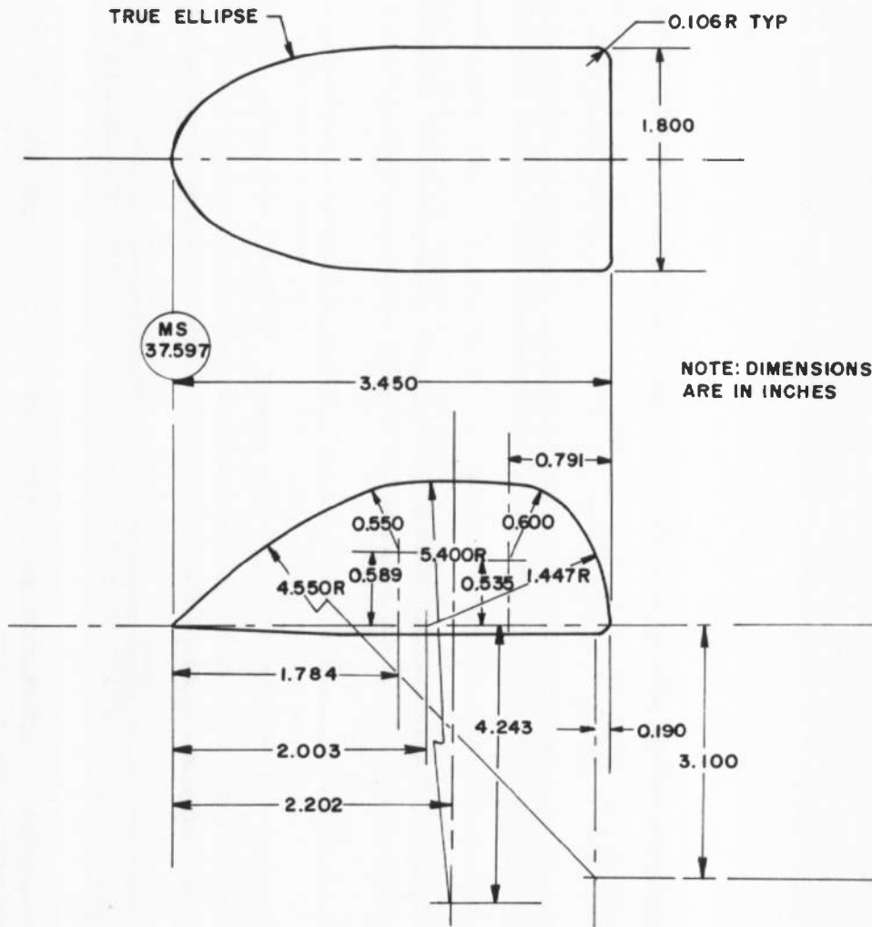
g. Horizon-Sensor Fairing Fig. 4 Concluded
