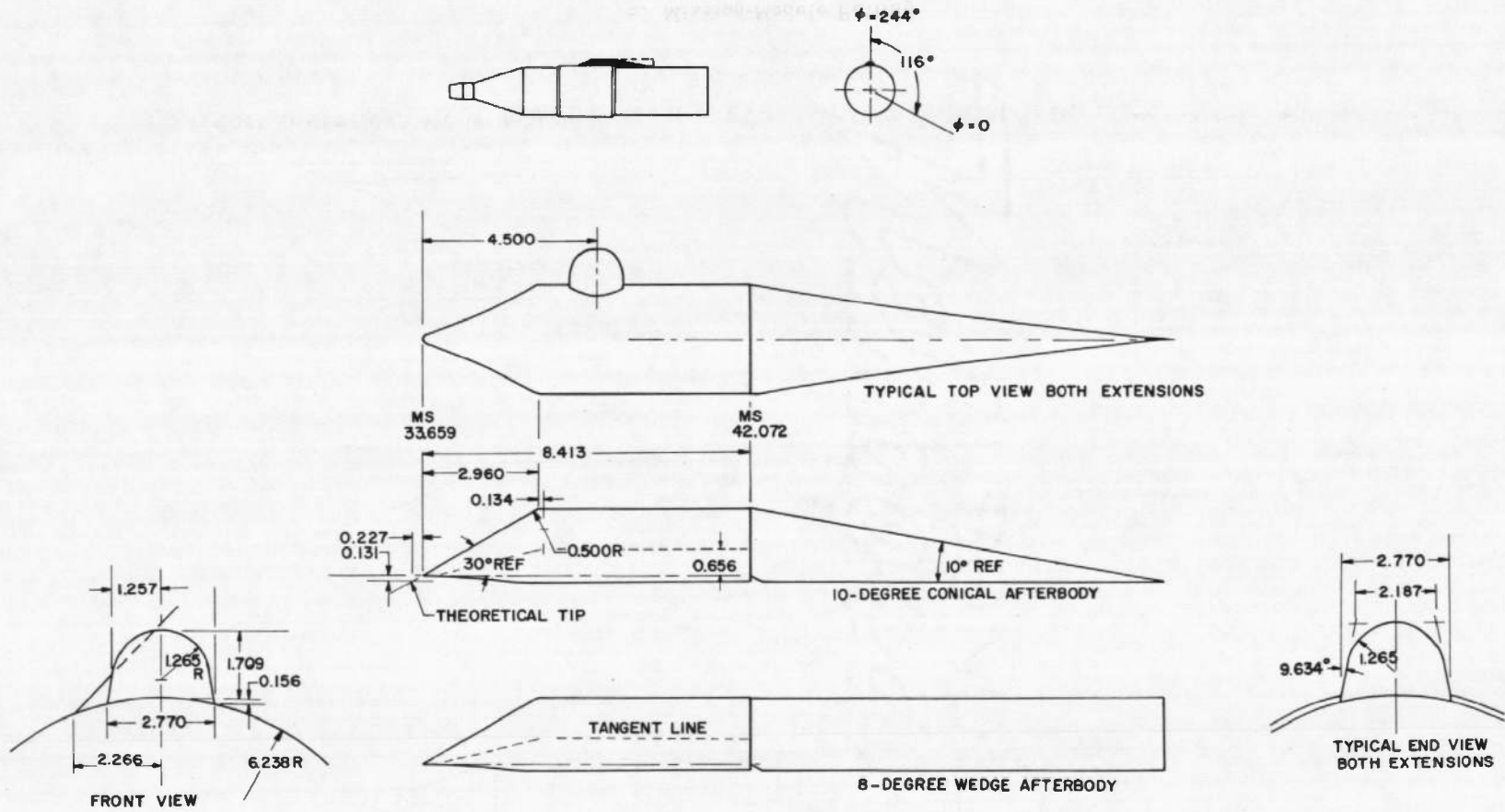
d. Left-Side Auxiliary-Equipment Fairing with 10-deg Cone and 8-deg Wedge Afterbody Fig. 4 Continued
