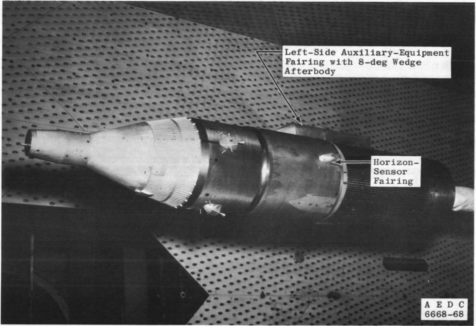
d. Configuration 3, Right-Side Auxiliary-Equipment Fairing Removed Fig. 5 Continued
