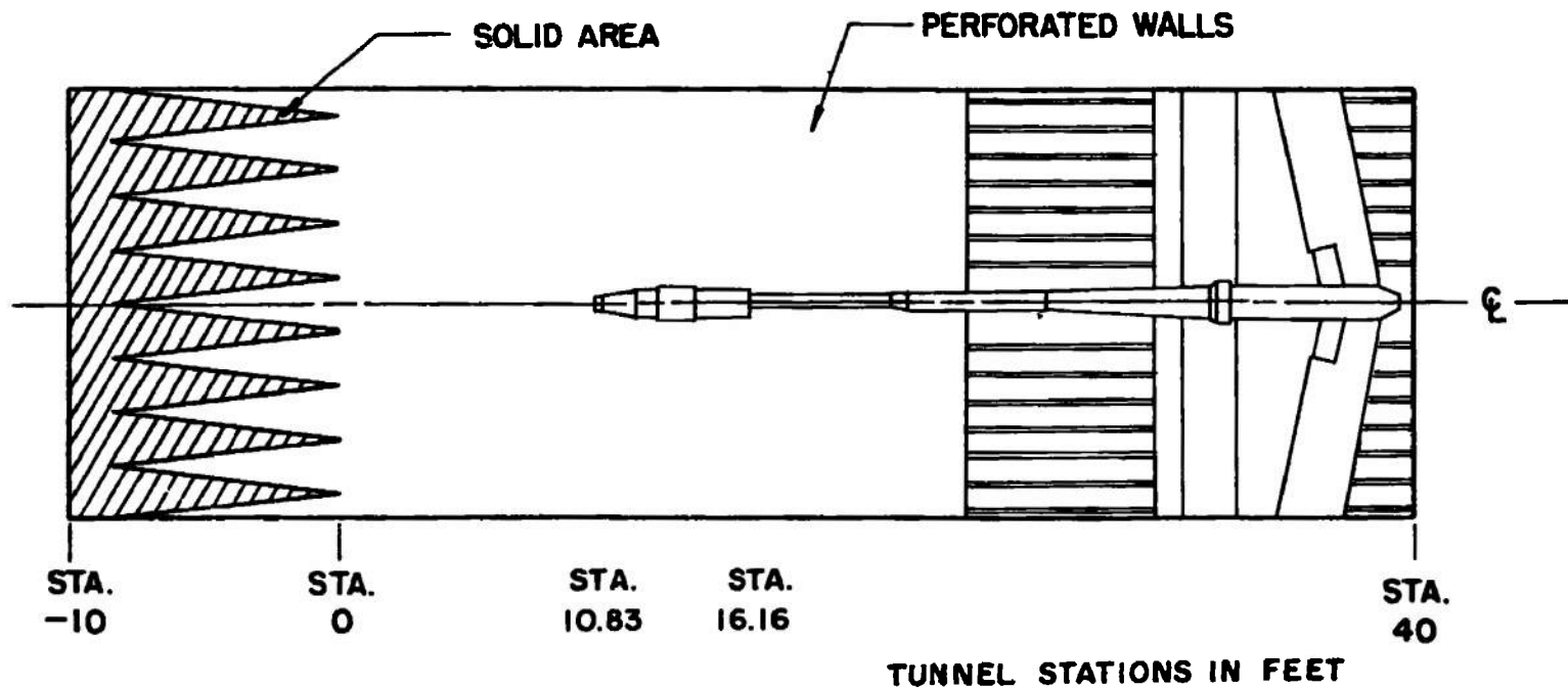
Fig. 1 Schematic of the MOL Fluctuating-Pressure Model in 16T Test Section
