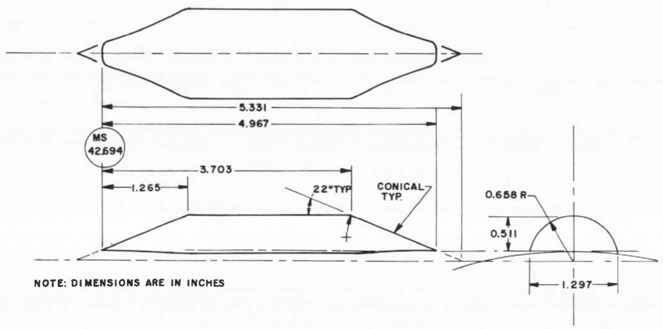
c. Mission-Module Foiring Fig. 4 Continued
