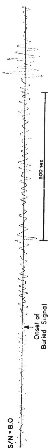
Figure 6. Examples of the synthetic seismograms at various S/N ratios from the subarray AO.
