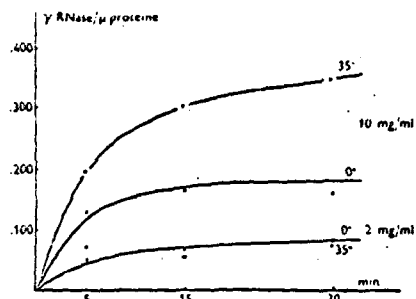
Fig. 4. Penetration of RNase- ^{131}\text{I} into ascites tumor cells as a function of the concentration of the enzyme, 2 and 10 mg/ml of suspended cells, and as a function of incubation temperature 0°-35°C.
