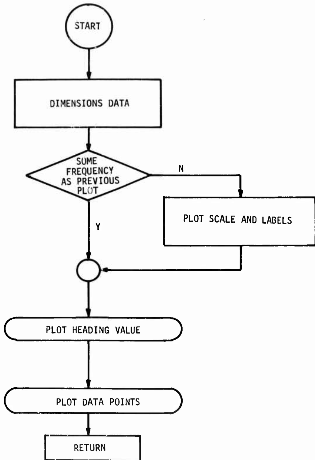
Figure 11. Block Diagram - Program DATAVE Subroutine PLOT
