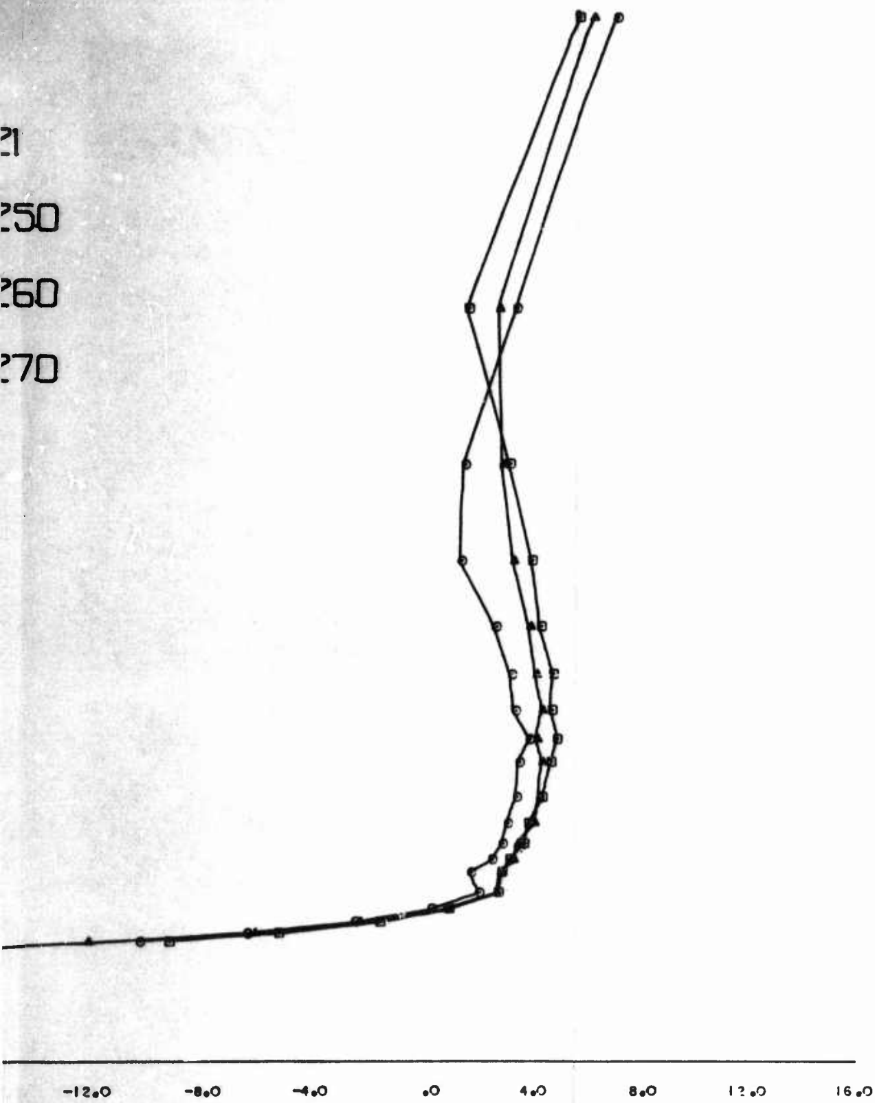
Figure 45. Iceland Antenna Patterns - 21 MHz
