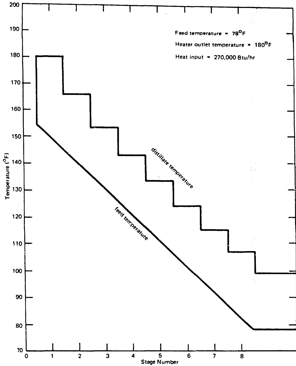
Figure 14. Temperature profile.
