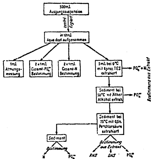
Figure 1 - Schema for fractionation procedures (see methods)
