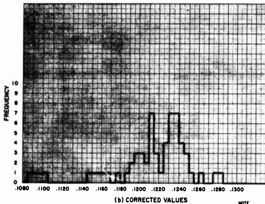
Figure 7-8 Histograms for Distance Measurements Made September 14, 1967
