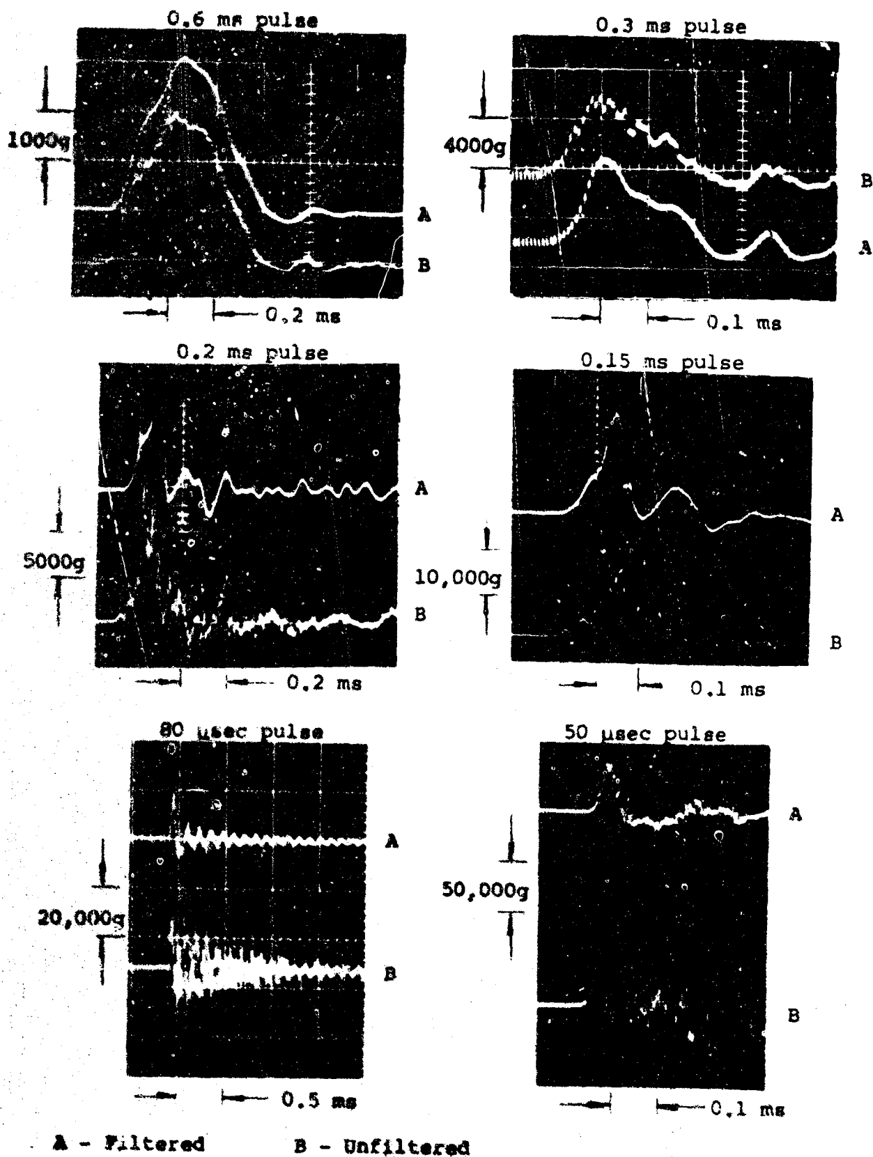
FIG. B-2. MECHANICAL FILTER RESPONSE TO SHORT IMPACTS
