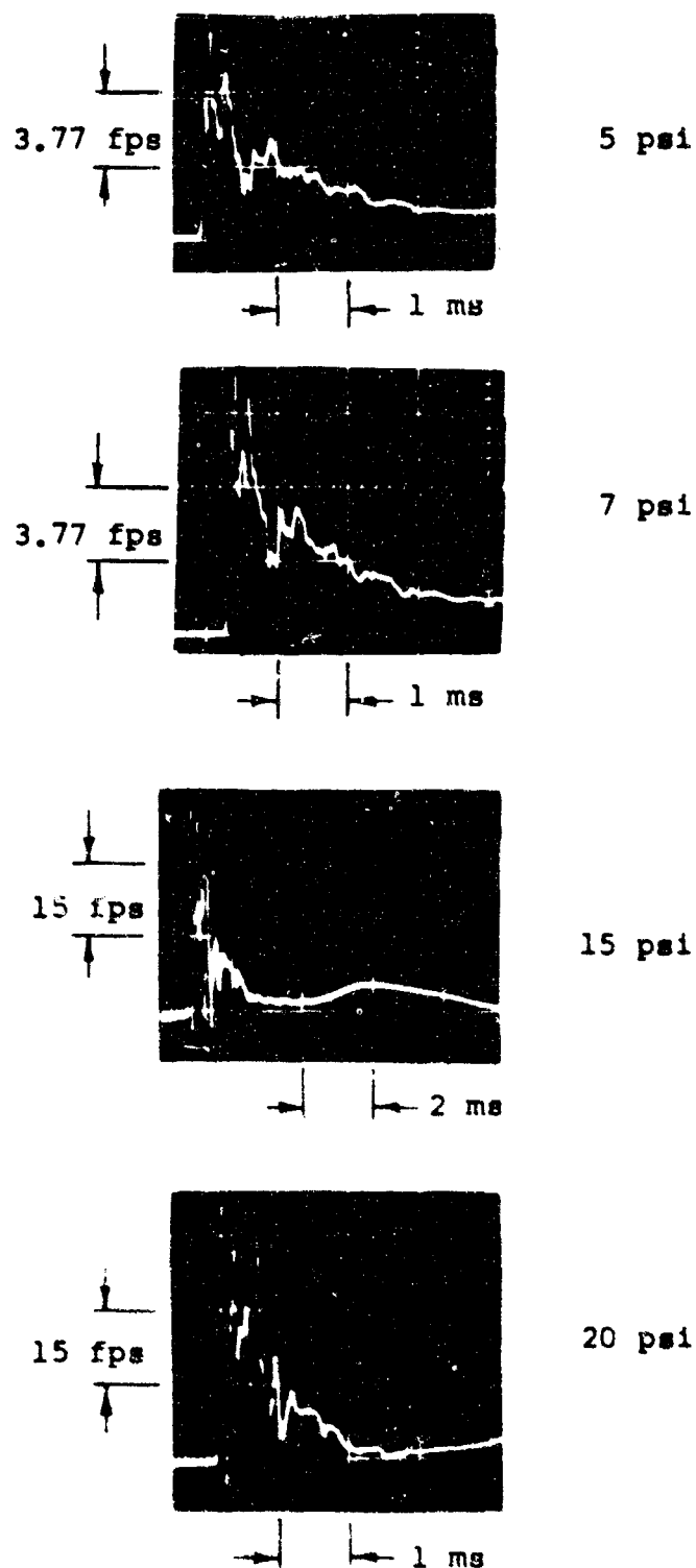
FIG. B-7. SAMPLE VELOCITY OSCILLOGRAMS (10-1b Payload)
