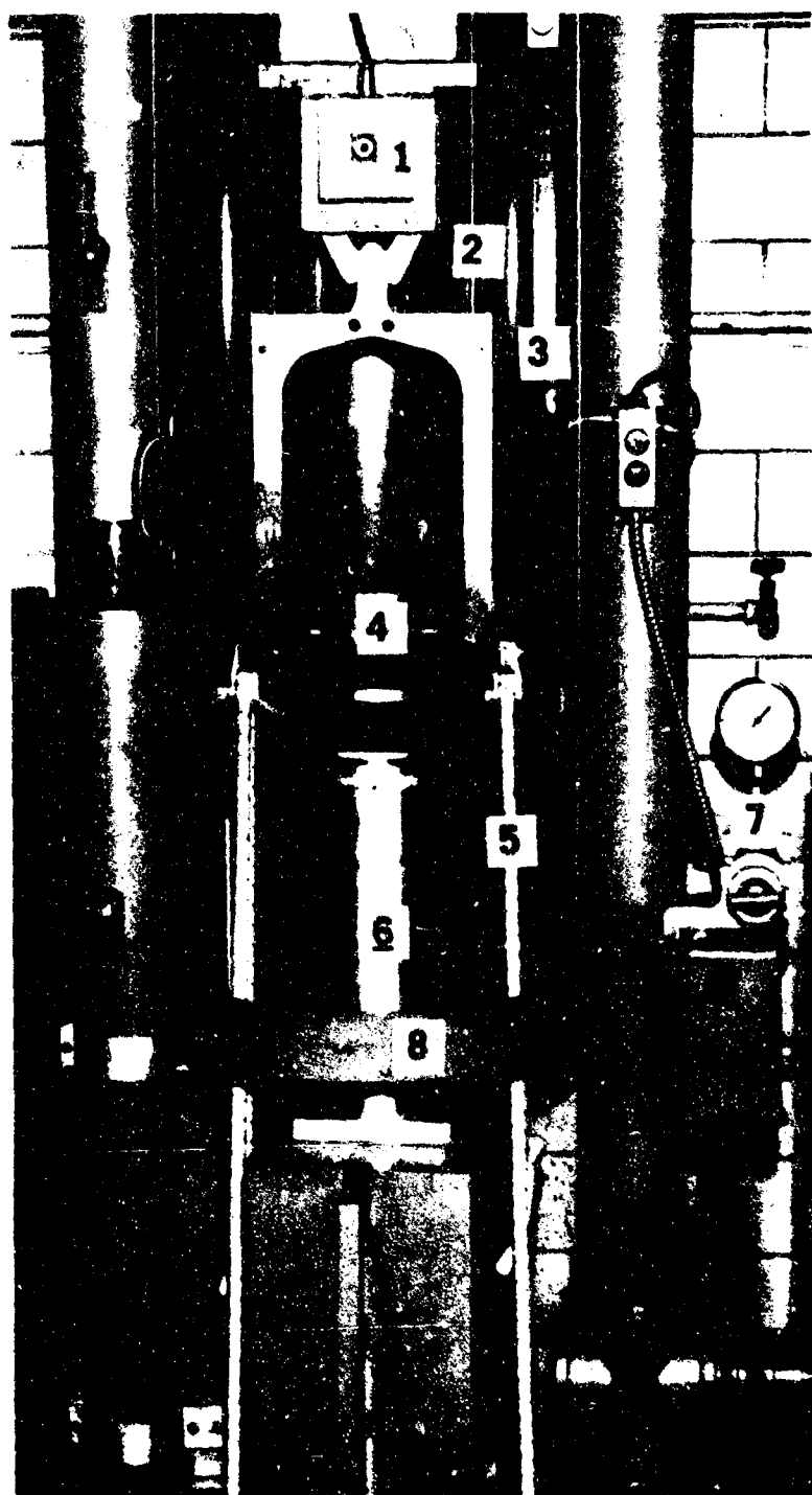
FIG. A-1. MK 7 MODIFICATIONS FOR FEASIBILITY STUDIES
