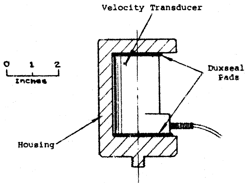
FIG. B-1. MECHANICAL FILTERS FOR ACCELEROMETER AND VELOCITY TRANSDUCER
