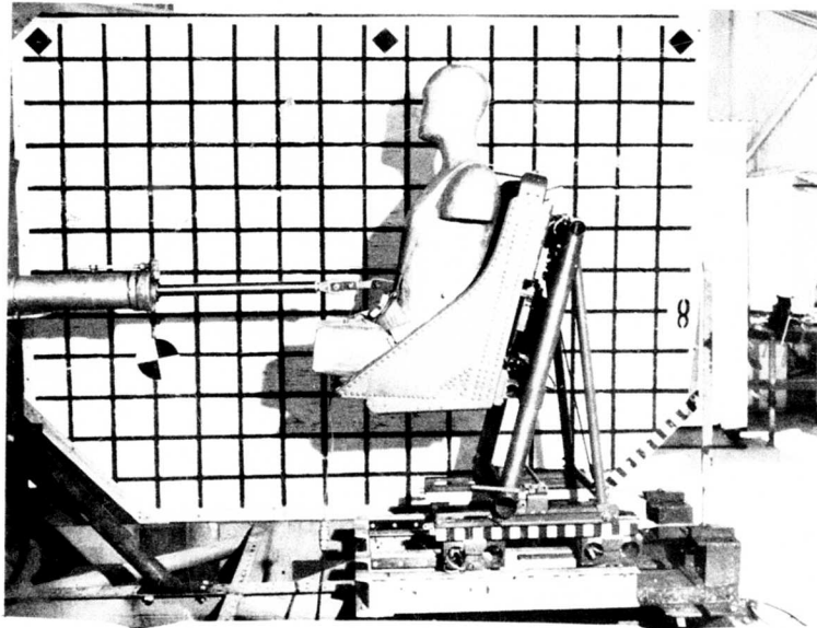
Figure 10. Test Setup for Longitudinal Static Test.
