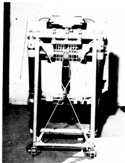
Figure 4. Rear View - Hayes Armored Aircrew Survival Seat.
