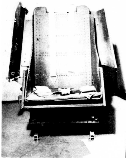
Figure 3. Front View - Hayes Armored Aircrew Survival Seat.
