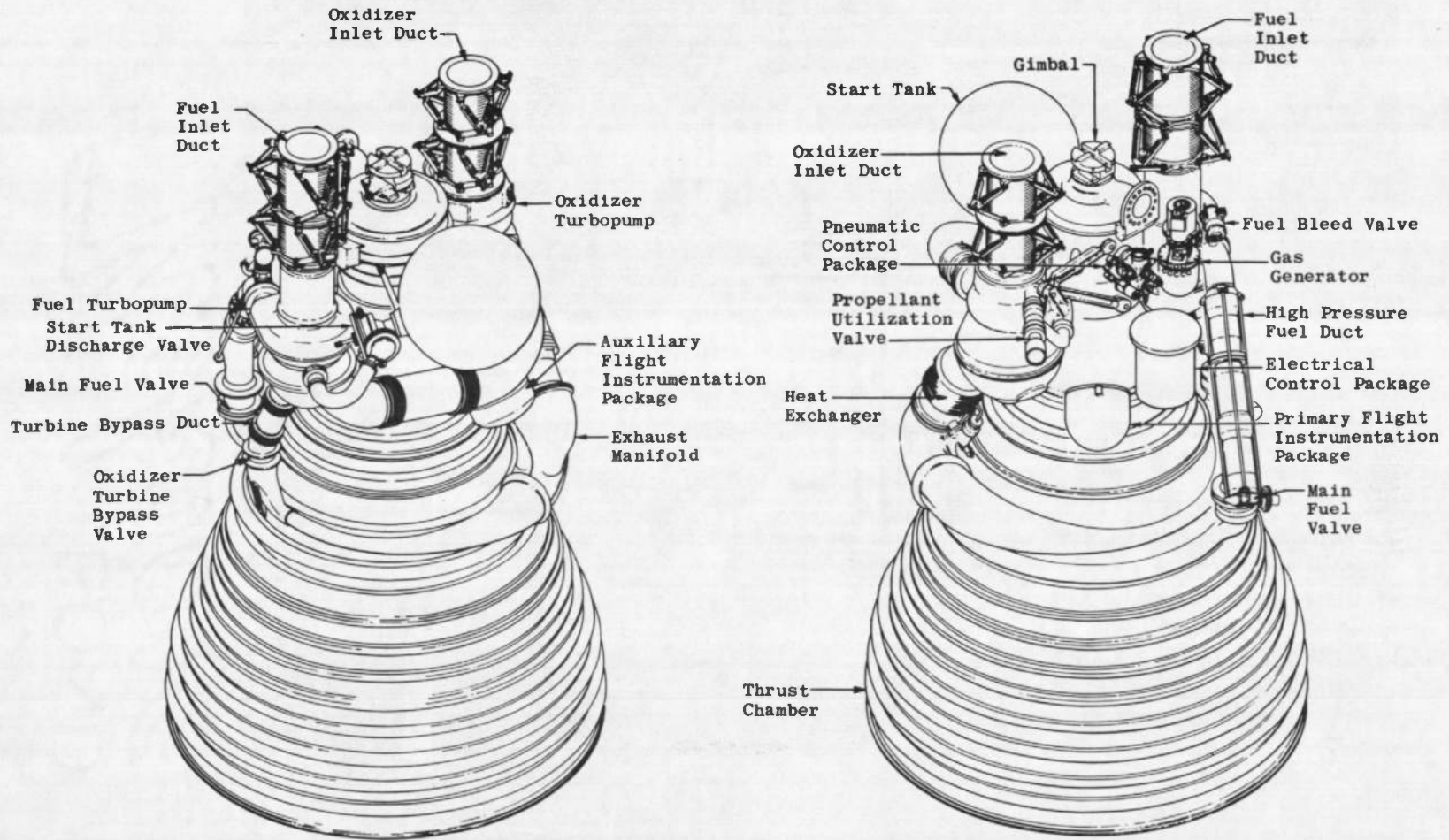
Fig. 3 Engine Details
