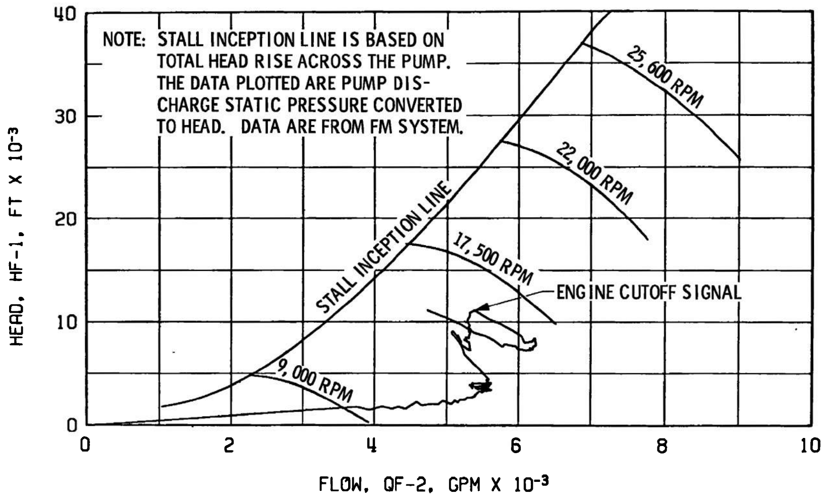
Fig. 35 Fuel Pump Start Transient Performance, Firing 38B
