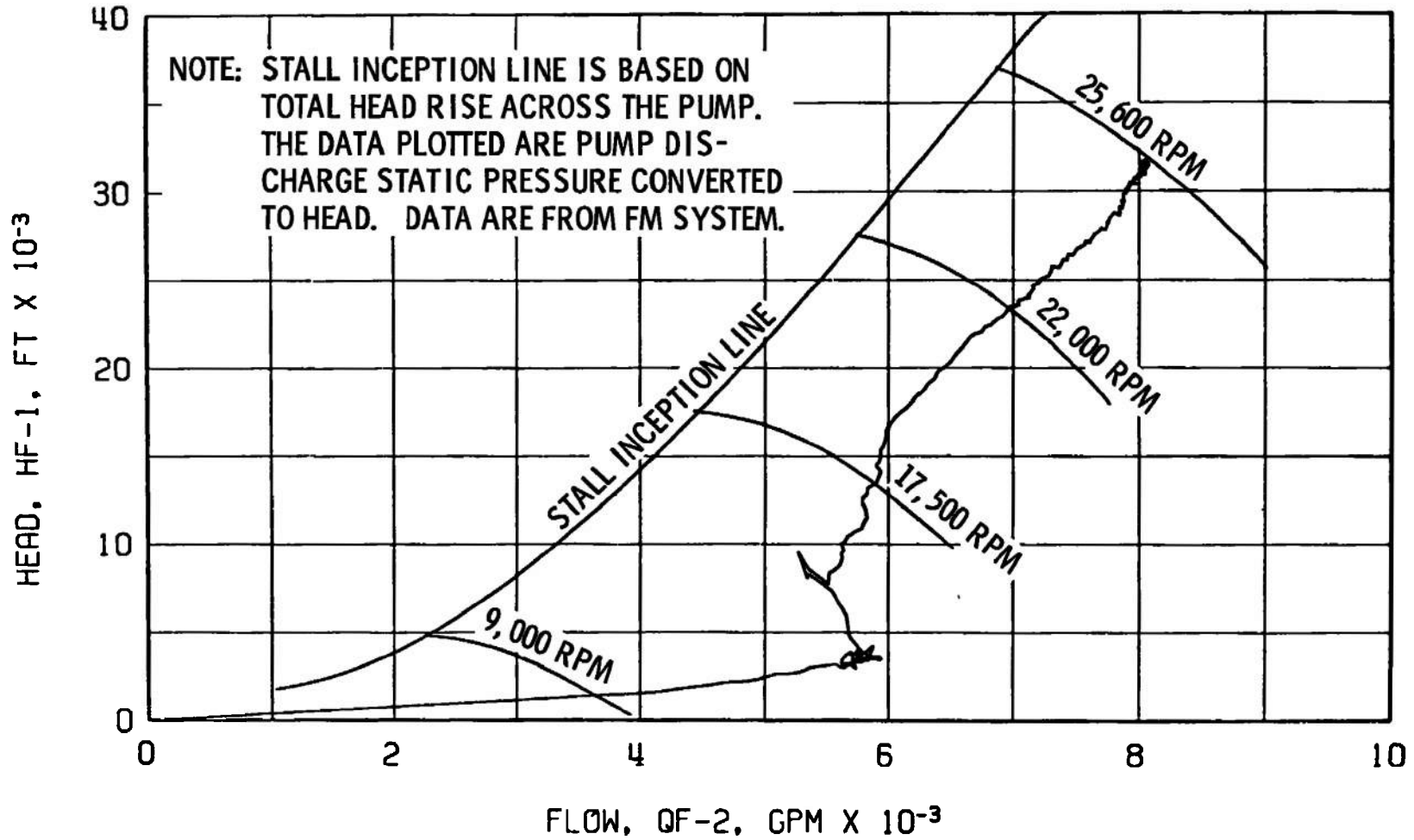
Fig. 23 Fuel Pump Start Transient Performance, Firing 37D
