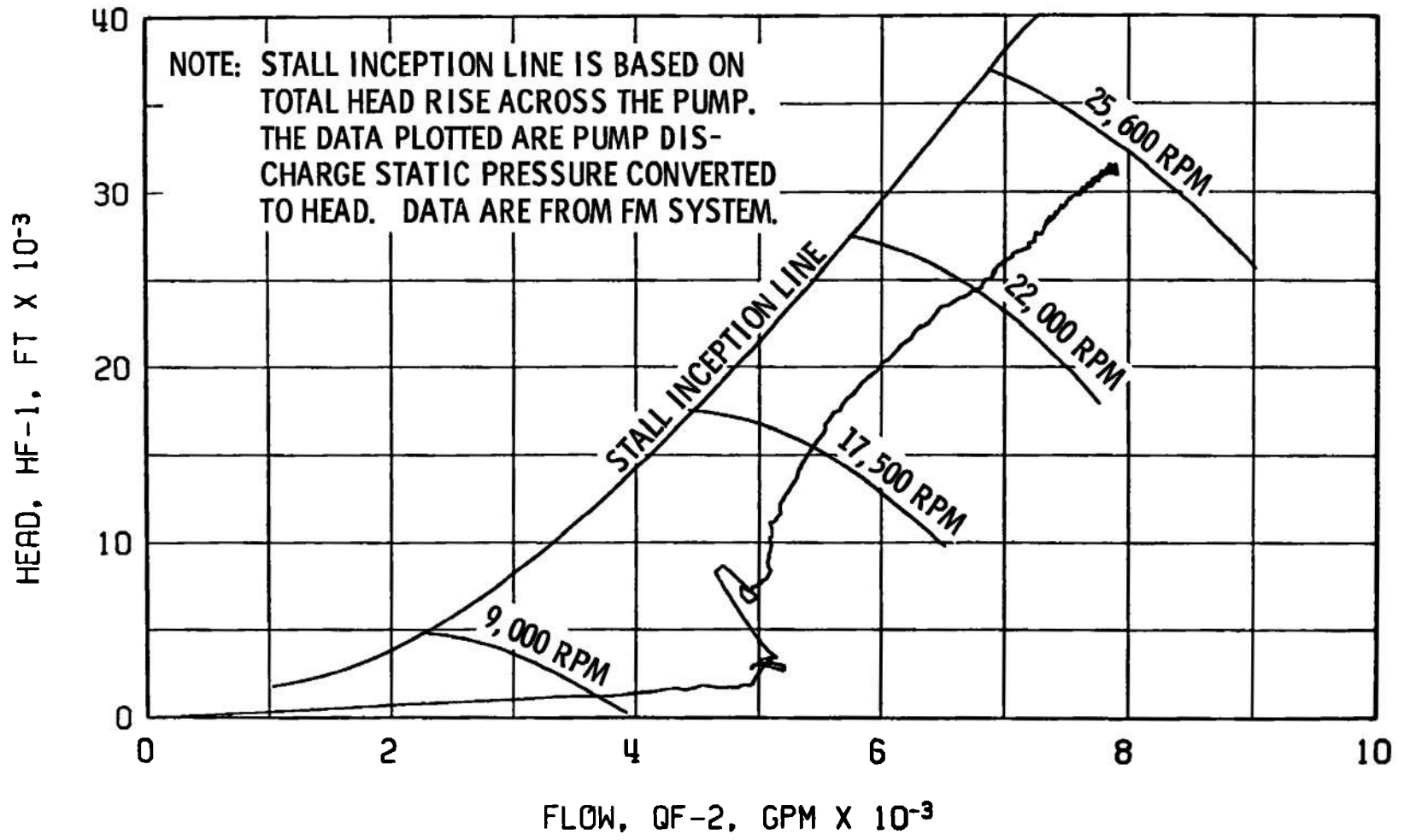
Fig. 15 Fuel Pump Start Transient Performance, Firing 37B
