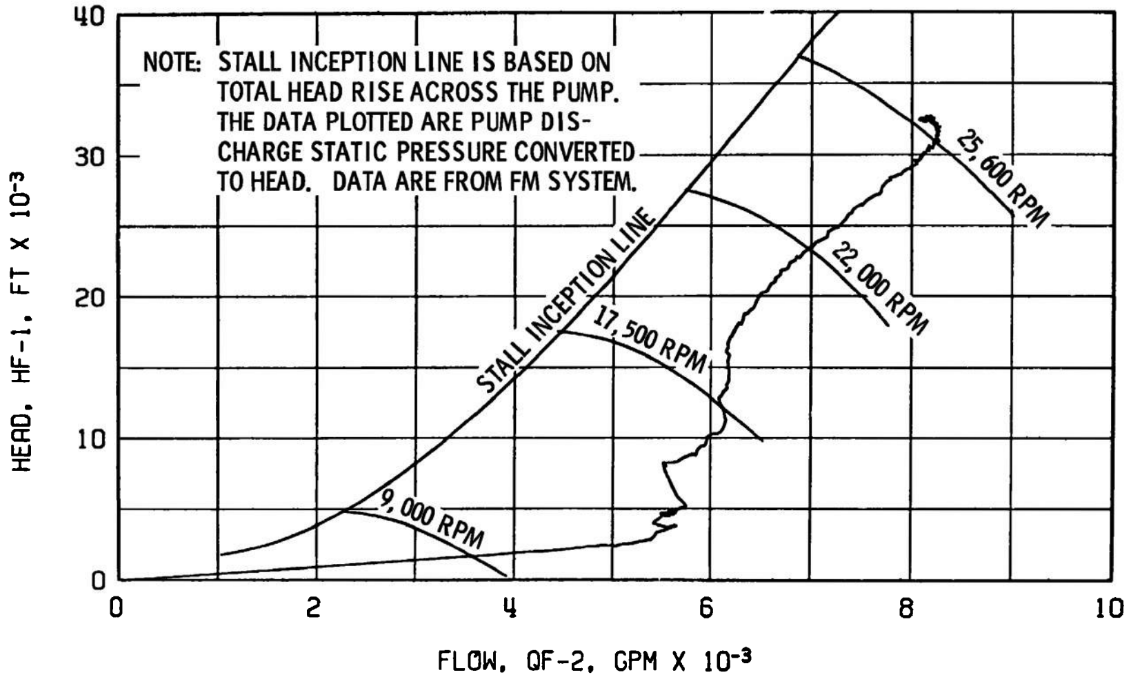
Fig. 43 Fuel Pump Start Transient Performance, Firing 38D
