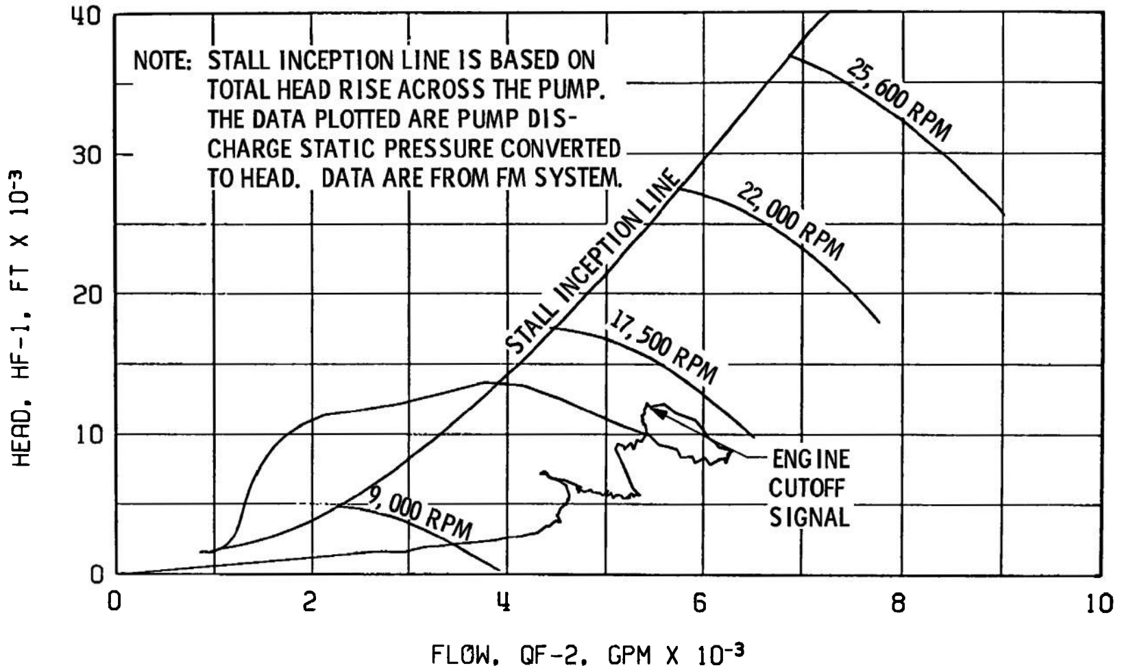
Fig. 27 Fuel Pump Start Transient Performance, Firing 37E
